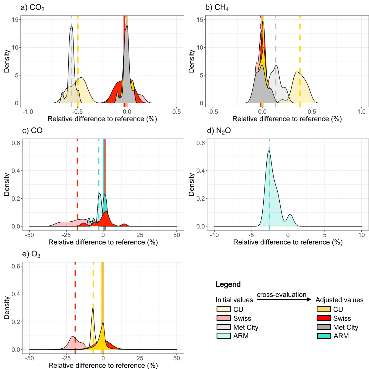
Fig. 4 Cross-evaluation of redundant measurements. Comparison of minute-averaged (a) CO 2 , (b) CH 4 , (c) CO and (d) N 2 O mole fractions measured in the University of Colorado (CU), Swiss, and Atmosphere Radiation Measurement (ARM) Program containers against atmospheric abundances inferred from discrete whole air sampling for post-cruise analysis at NOAA Global Monitoring Laboratory (used as calibration reference). (e) Comparison of minute-averaged O 3 mole fractions measured in the CU and Swiss containers against mole fractions measured in the ARM container (used as calibration reference). Shaded and solid contours show initial and adjusted (after cross-evaluation) values, respectively. The shape of the density distributions may change due to the use of time-dependent correction factors. Vertical dashed and solid lines show the median relative difference to the reference for initial and adjusted values, respectively. Note that the ARM N 2 O time series was not adjusted for calibration bias as we did not generate a merged N 2 O dataset. The kernel density estimates (smoothed version of a histogram) were computed using R package ggplot2 (version 3.3.3).
