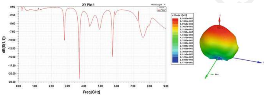
Fig. 8 Operating frequency and radiated pattern of RFID TAG designed with NUTL2
