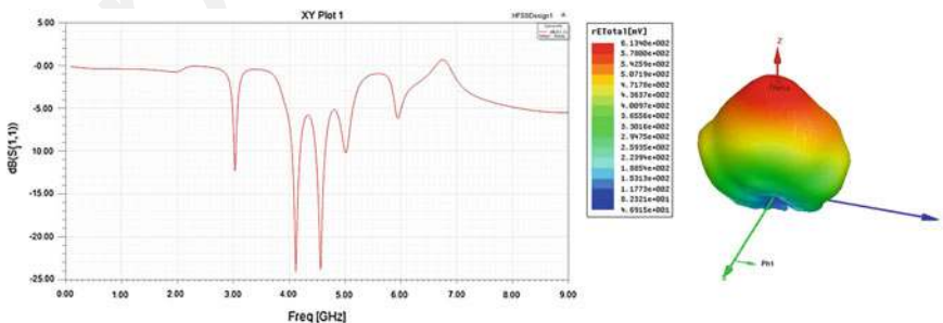
Fig. 6 Operating frequency and radiated pattern of RFID TAG designed with LNUT1
