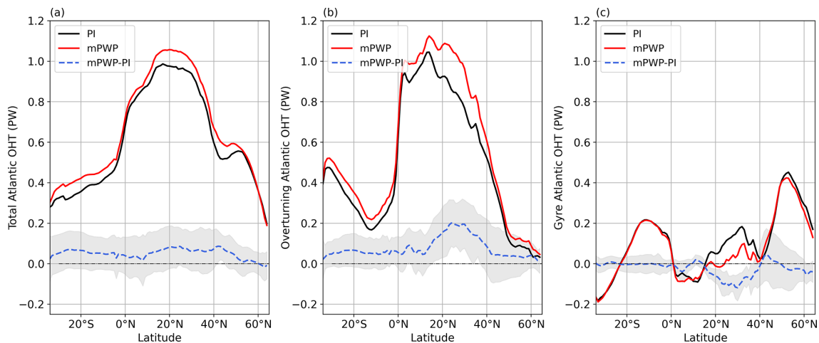
Figure 10. (a) MMM total Atlantic Ocean heat transport in the mid-Pliocene and pre-industrial and the difference. (b) MMM Atlantic Ocean heat transport by overturning. (c) MMM Atlantic Ocean heat transport by wind-driven gyres. The shading indicates 1 standard deviation by individual models from the MMM.
