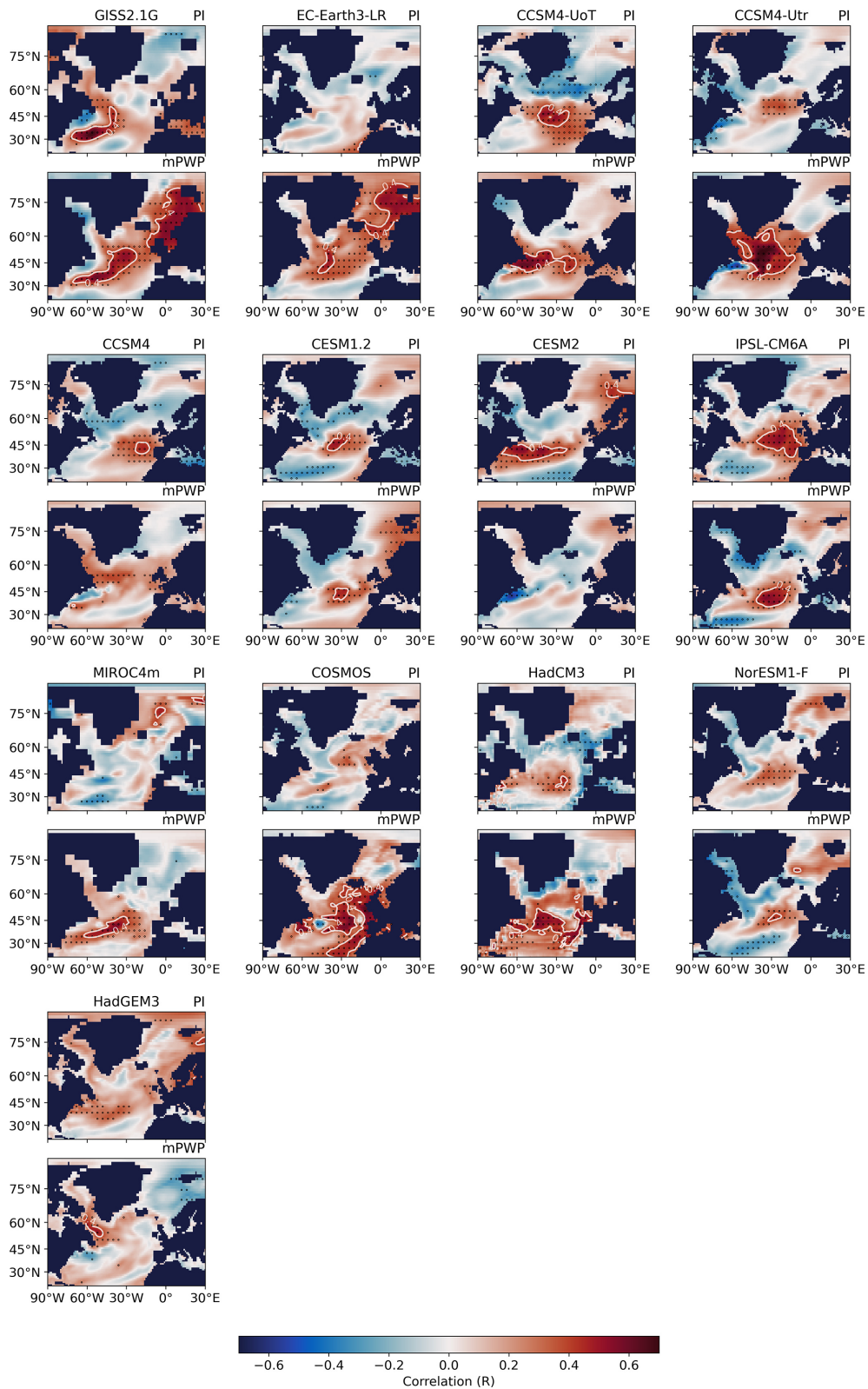
Figure 3. Correlation between the annual AMOC strength and annual SSTs for individual models. The top panel for each model shows the results for the pre-industrial, and the bottom panel shows the results for the mid-Pliocene. Both the AMOC strength and SSTs have been linearly detrended before correlating. Stippling indicates significance at the 95 % confidence level. White contours show a positive correlation of R = 0.4 .
