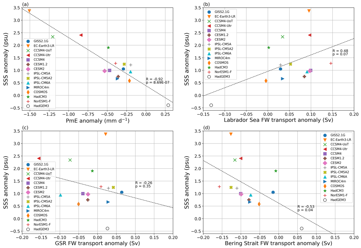
Figure 9. The mPWP–PI change in sea surface salinity plotted against (a) the mPWP–PI change in PmE freshwater flux, (b) the mPWP–PI change in northward freshwater transport at the northern boundary of the Labrador Sea (62° N), (c) the mPWP–PI change in northward freshwater transport across the GSR (62° N) and (d) the mPWP–PI change in northward freshwater transport across the Bering Strait. The sea surface salinity and PmE anomalies are averaged over the eastern subpolar North Atlantic and Labrador Sea (45–60° N, 30–60° W); the area indicated by the blue box in Fig. 6b).
