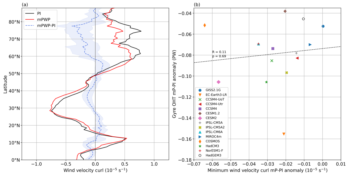
Figure 12. (a) MMM Atlantic zonal-mean 1000 hPa wind velocity curl ( \frac{dv}{dx} - \frac{du}{dy} ) in the pre-industrial and mid-Pliocene and their difference. Shading indicates 1 standard deviation from the MMM difference by individual models. (b) The minimum zonal-mean 1000 hPa wind velocity curl between 20–40° N plotted against the 20–40° N average OHT gyre component anomaly for individual models.
