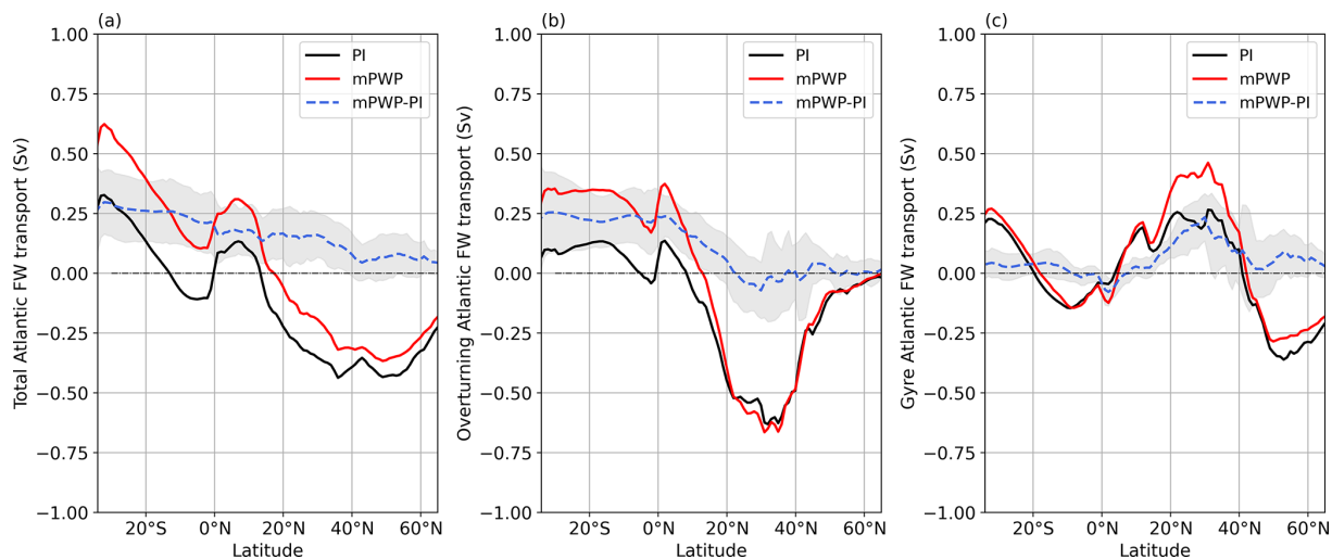
Figure 7. (a) MMM total Atlantic freshwater transport in the mid-Pliocene and pre-industrial and the difference. (b) MMM Atlantic freshwater transport by overturning. (c) MMM Atlantic freshwater transport by wind-driven gyres. The shading indicates 1 standard deviation of deviation from the MMM difference by individual models.
