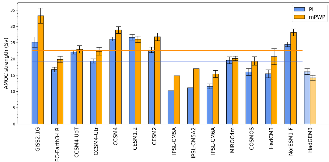
Figure 1. Individual model AMOC strength in the pre-industrial (blue) and mid-Pliocene (orange). Error bars indicate 1 standard deviation from the time-mean AMOC strength computed using 100 years of annual data. The horizontal lines indicate the multi-model mean AMOC strength.
