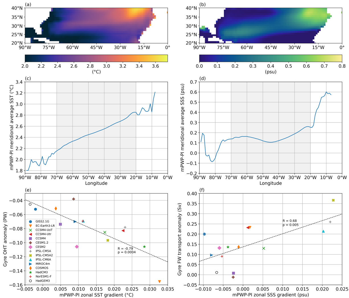
Figure 13. (a) MMM mPWP–PI Atlantic SST difference between 20–40° N. (b) MMM mPWP–PI Atlantic SSS difference between 20–40° N. (c) MMM 20–40° N meridional-mean mPWP–PI Atlantic SST difference. (d) MMM 20–40° N meridional-mean mPWP–PI Atlantic SSS difference. (e) Individual model mPWP–PI mean difference in zonal SST gradient from (c) between 20–70° W plotted against the mPWP–PI difference in the OHT gyre component. (f) Individual model mPWP–PI mean difference in the zonal SSS gradient from (d) between 20–70° W plotted against the mPWP–PI difference in the gyre freshwater transport.
