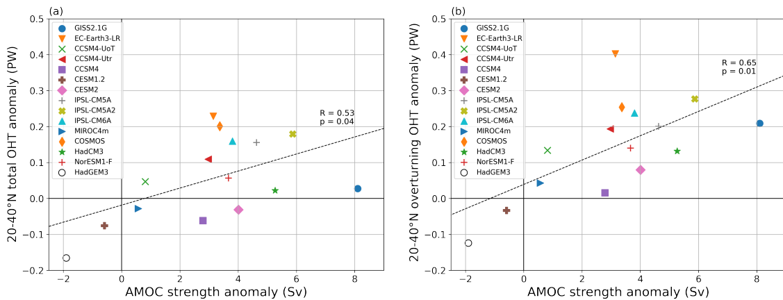
Figure 11. (a) The mPWP–PI change in average total Atlantic OHT between 20–40° N and change in AMOC strength. (b) The mPWP–PI change in overturning Atlantic OHT between 20–40° N and change in AMOC strength. The dotted line indicates a linear fit by least squares with the correlation coefficient R and p value of fit shown.
