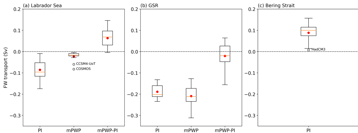
Figure 8. Boxplots of the mean freshwater transport (Sv) in the pre-industrial and mid-Pliocene and their difference at 62^{\circ} N (a) near the northern boundary of the Labrador Sea and (b) across the GSR. (c) Mean freshwater transport (Sv) through the Bering Strait in the pre-industrial. The box covers Q1 (25th percentile) to Q3 (75th percentile), with the median indicated by a horizontal orange line. The whiskers extend from Q1 to Q1 - 1.5 \times \text{IQR} (interquartile range) and from Q3 to Q3 + 1.5 \times \text{IQR} , where \text{IQR} = Q3 - Q1 . A model that falls outside the whiskers is separately shown as an unfilled circle. The MMM is indicated by a filled red circle.
