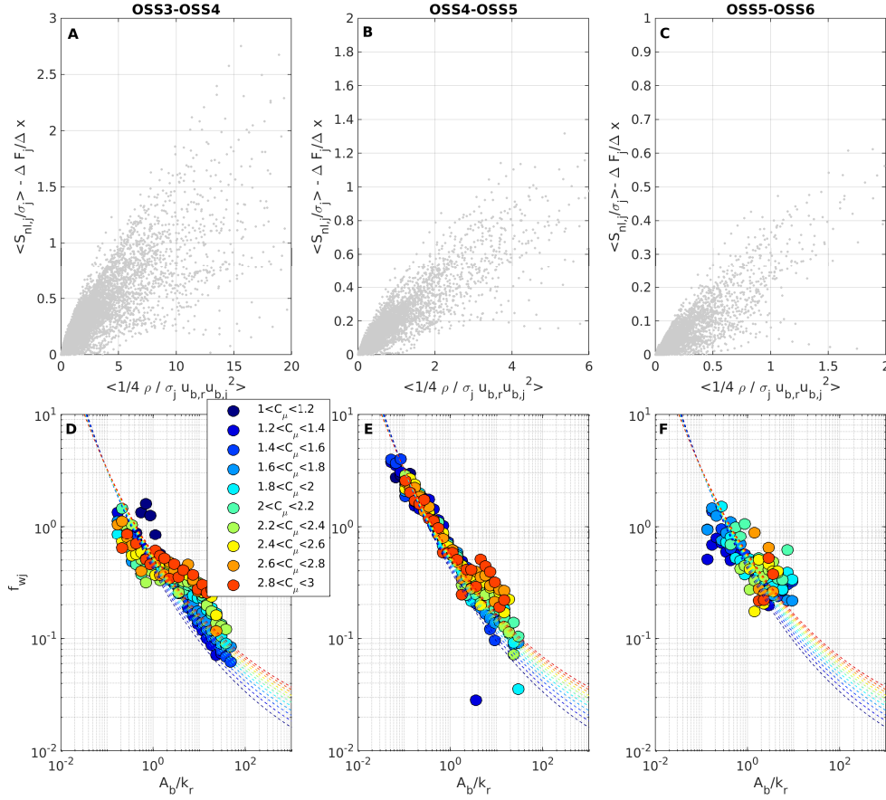
Figure 3. Top: Dissipation estimated from the observed action flux gradient \langle \epsilon_{f,j}/\sigma_j \rangle = \langle S_{nl,j}/\sigma_j \rangle - \Delta F_j/\Delta x as a function of \langle \epsilon_{f,j}/\sigma_j \rangle / f_{e,j} = 1/4 \langle \rho/\sigma_j u_{b,r} u_{b,j}^2 \rangle according to Madsen (1995)'s parameterization over OSS3-OSS4, OSS4-OSS5 and OSS5-OSS6 barrier sections. Bottom: Wave friction factor f_{w,j} vs the ratio between near-bed wave excursion A_b and bed roughness k_r for the binned field data (colored circles) and the predictions from Madsen's formulation (Madsen, 1995) (dashed lines). The color levels refer to the value of C_\mu factor.
