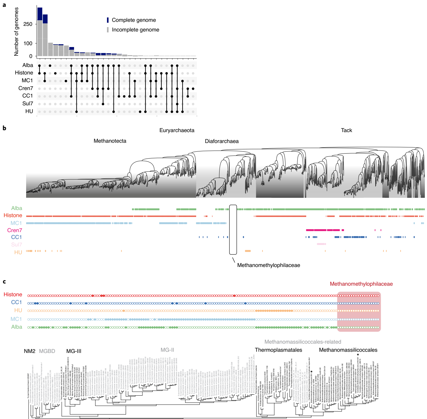
Fig. 1 Distribution of NAPs across archaea. a , Co-occurrence of previously characterized archaeal NAPs in 1,419 sequenced archaeal genomes. b , Presence/absence of NAPs in phylogenetic context, highlighting the Methanomethylphilaceae as a family without any previously characterized NAPs. For species-level information, see Supplementary Table 1 and Supplementary Fig. 1. c , NAPs in the Diaforarchaea. Presence/absence of
