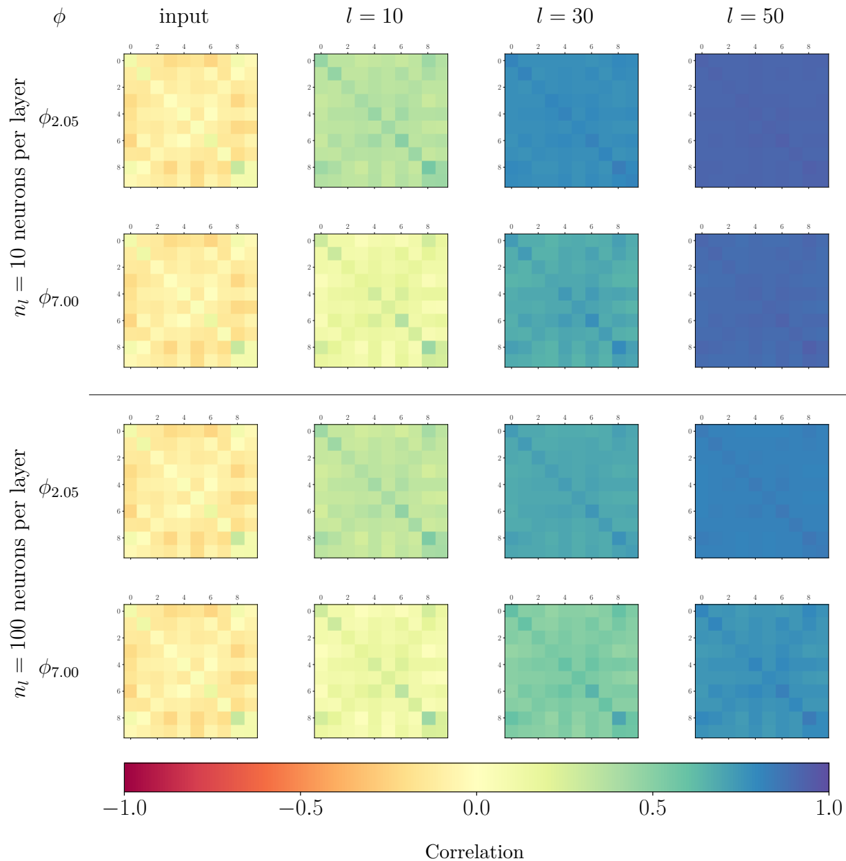
Figure 15: Propagation of correlations c_{ab}^l in a multilayer perceptron with activation function \phi_{\theta} with \theta \in \{2.05, 7.00\} and inputs sampled from the CIFAR-10 dataset. The weights are sampled from \mathcal{W}(\theta, 1) and the biases are zero. Each plot displays a 10 \times 10 matrix C_{pq}^l whose entries are the average correlation between the pre-activations propagated by samples from classes p, q \in \{0, \dots, 9\} , at the input and right after layers l \in \{10, 30, 50\} .
