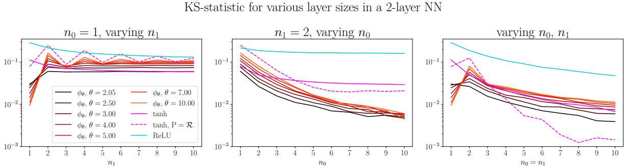
Figure 11: Evolution of the distance of the standardized distribution of Z to the \mathcal{N}(0, 1) according to the Kolmogorov-Smirnov statistic. Weight initialization is \mathcal{W}(\theta, 1) when using \phi = \phi_\theta and is Gaussian according to the EOC when using \phi = \tanh or ReLU. For each point, we have computed the KS-statistic over 200 000 samples of (\mathbf{X}, \mathbf{W}^1, \mathbf{W}^2) .
