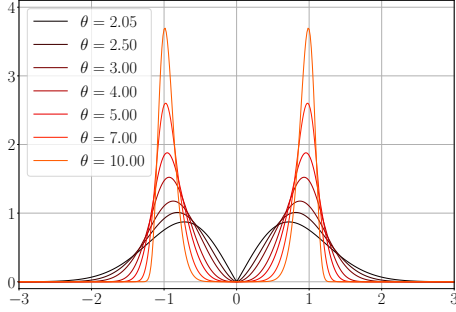
(a) Initialization distribution P_\theta of the weights: symmetric Weibull \mathcal{W}(\theta, 1) .
