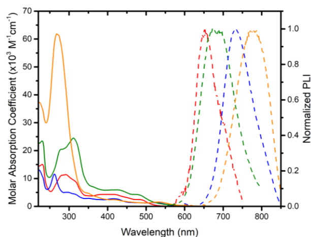
Figure 2. Absorption (solid line) and emission (dashed line) spectra of [Ru(phen) 2 (dph)] 2+ 1 (orange), [Ru(phen) 2 (bphh)] 2+ 2 (blue), [Ru(TAP) 2 (dph)] 2+ 3 (green) and [Ru(TAP) 2 (bphh)] 2+ 4 (red) in acetonitrile at room temperature.
