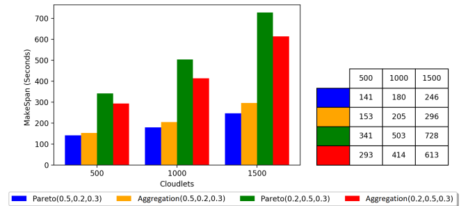
Fig. 1. Comparison of makespan with 30 VMs.
