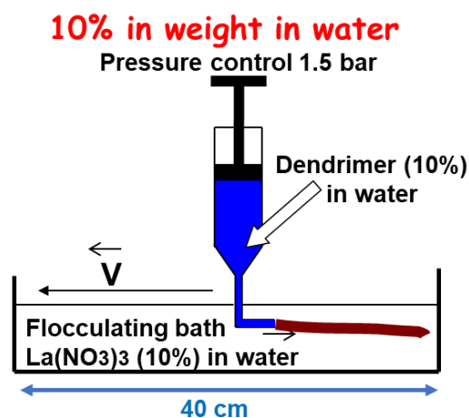
Figure 4. Schematization of the method used for producing dendrimer fibers with dendrimer 1a-G4 .
