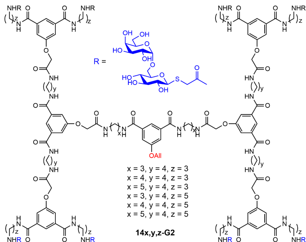
Figure 11. Structure of a large family of glycodendrons obtained by a parallel combinatorial approach and suitable for producing hydrogels at low concentration.
