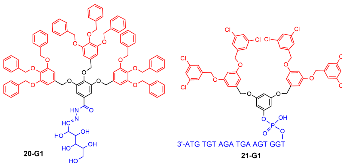
Figure 15. Structure of dendrons having a hydrophilic core and hydrophobic surface and branches.
