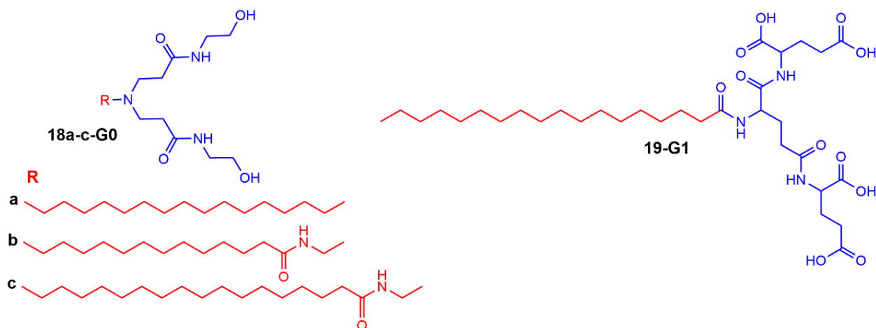
Figure 14. Amphiphilic dendrons having a long alkyl chain as their core.
