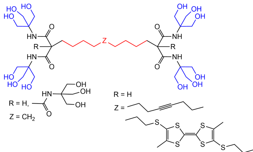
Figure 1. Structure of bolaform arborols suitable for forming hydrogels.
