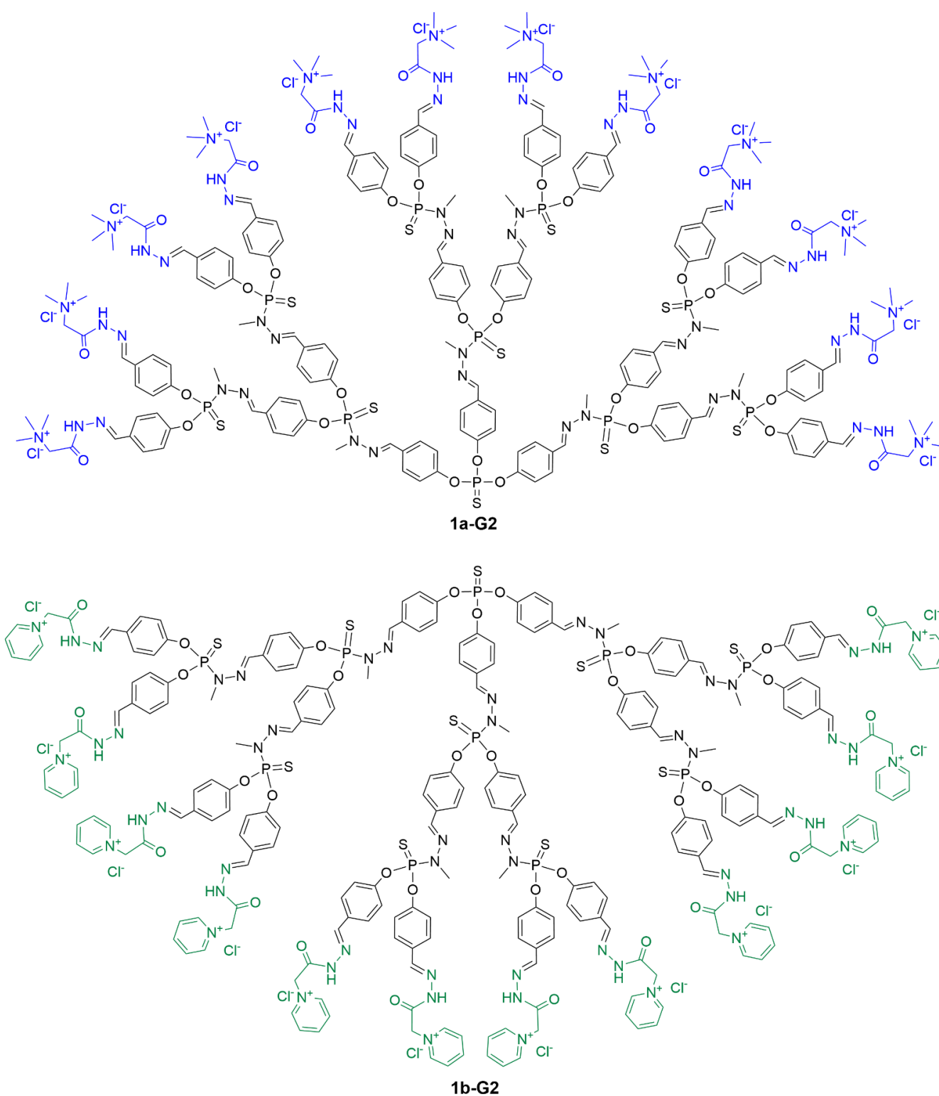
Figure 2. Full chemical structure of dendrimers 1a-G2 (functionalized with the Girard T reagent) and 1b-G2 (functionalized with the Girard P reagent).
