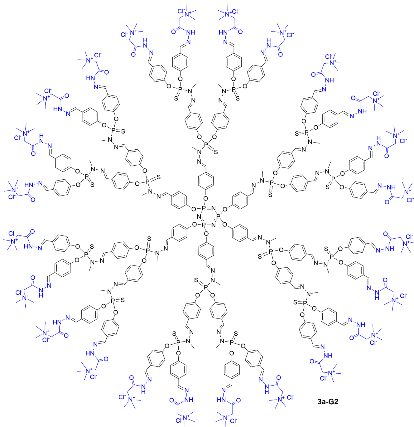
Figure 6. Full chemical structure of dendrimer 3a-G2.
