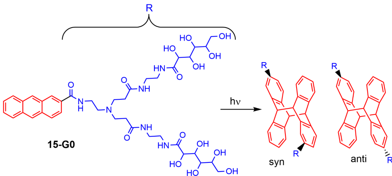
Figure 12. A small dendron having an anthracene at the core, able to dimerize under photo-irradiation.
