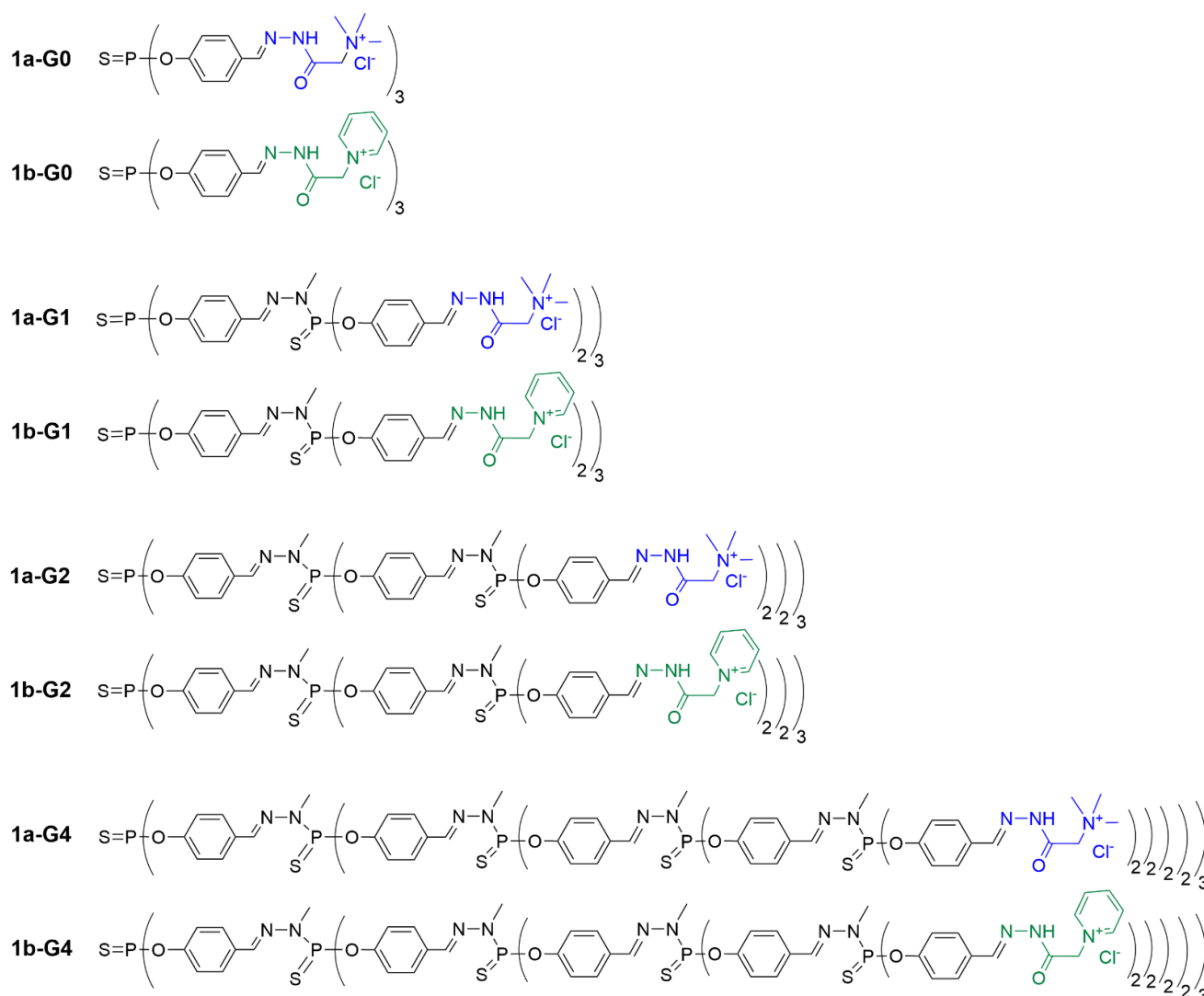
Figure 3. Linear representation of the chemical structure of phosphorus dendrimers built from a trifunctional core and functionalized with the Girard T reagent (series a , in blue) or the Girard P reagent (series b , in green) as hydrophilic terminal functions.
