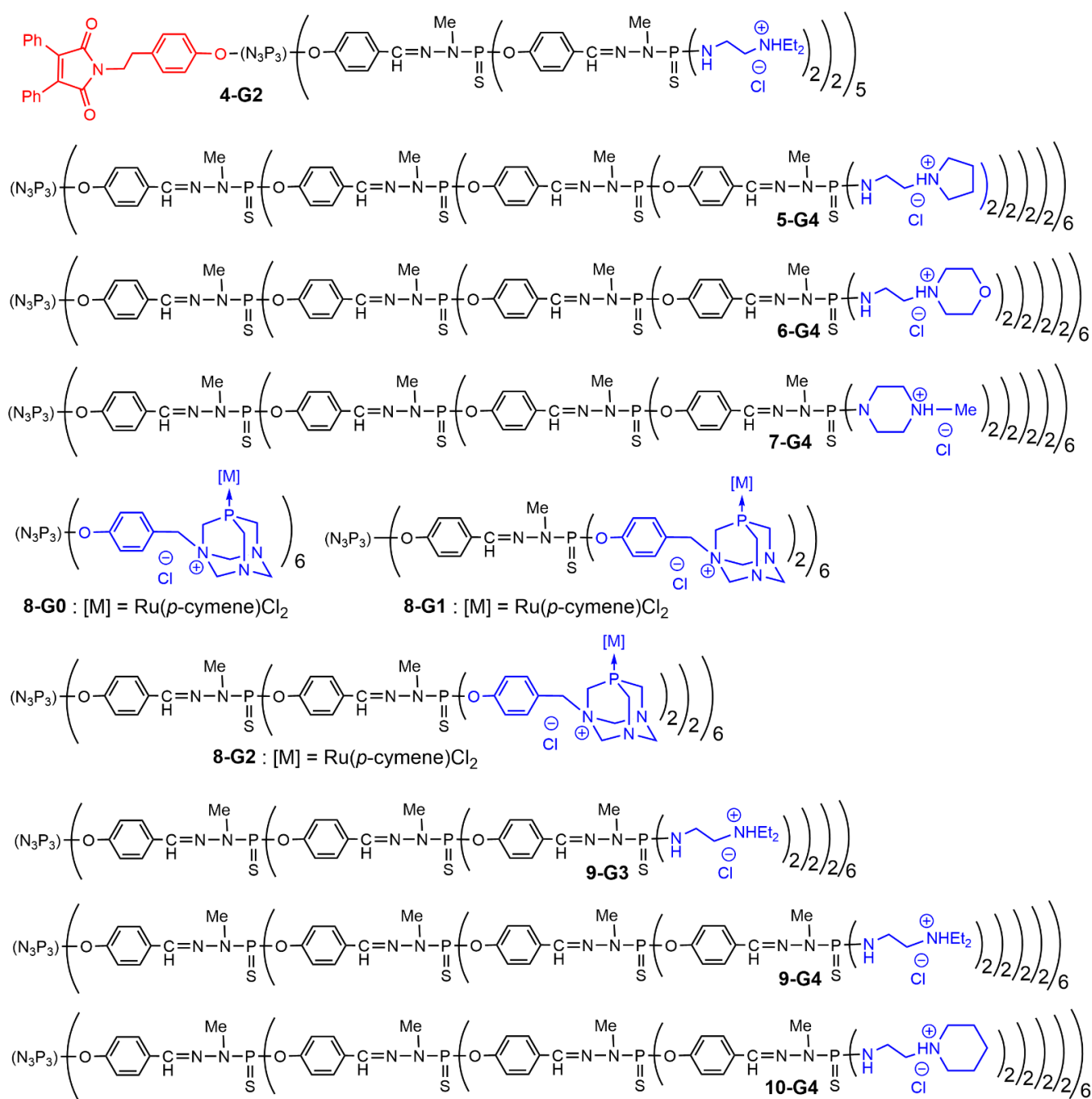
Figure 8. Structure of phosphorus dendrimers forming dendriplexes analyzed by agarose gel electrophoresis assays.
