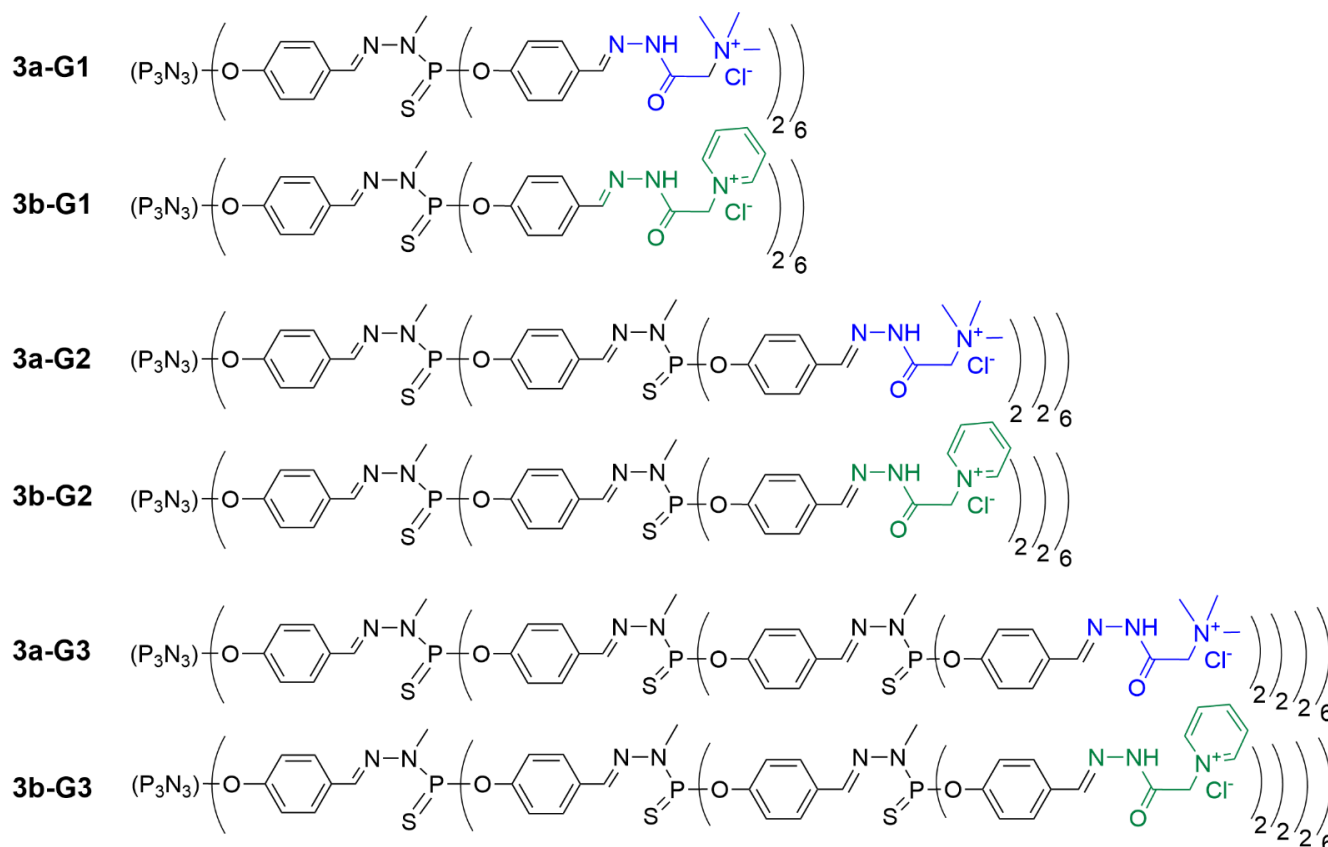
Figure 7. Linear representation of phosphorus dendrimers built from a hexafunctional core and functionalized with the Girard T reagent (in blue) or the Girard P reagent (in green) as terminal groups.
