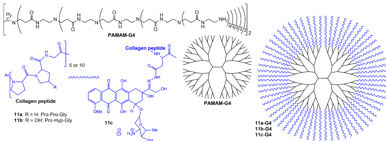
Figure 9. PAMAM dendrimers functionalized with collagen mimetics.
