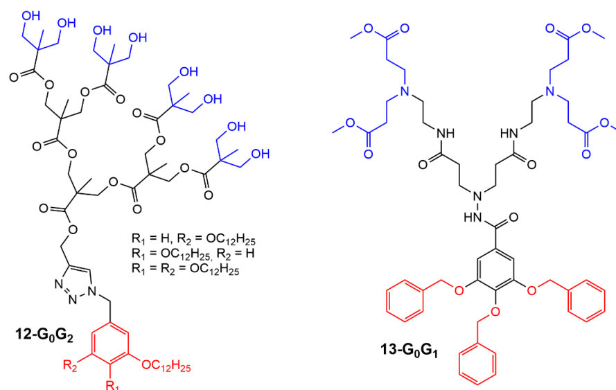
Figure 10. Structure of small amphiphilic Janus dendrimers suitable for affording hydrogels.
