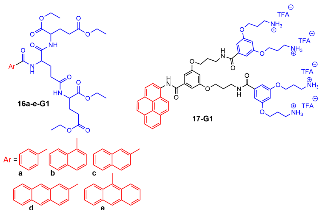
Figure 13. Examples of amphiphilic dendrons, for which the dendritic part is hydrophilic and the core is a lipophilic aromatic group.
