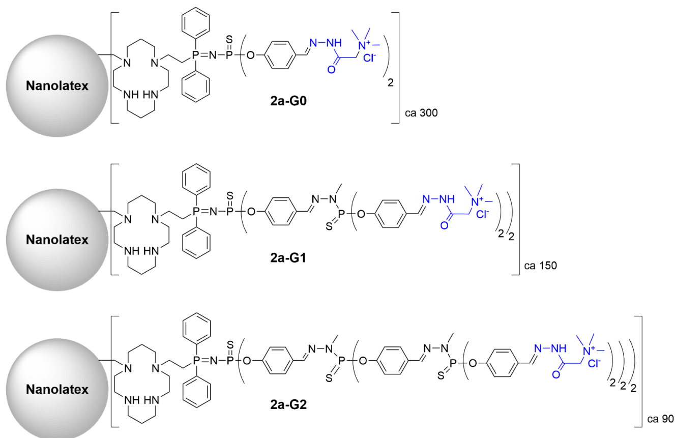
Figure 5. Nanolatex functionalized with phosphorus dendrons (generations 0 to 2) bearing the Girard T reagent as terminal functions. Cyclam moieties were suitable for the complexation of \text{Cu}^{2+} ions.
