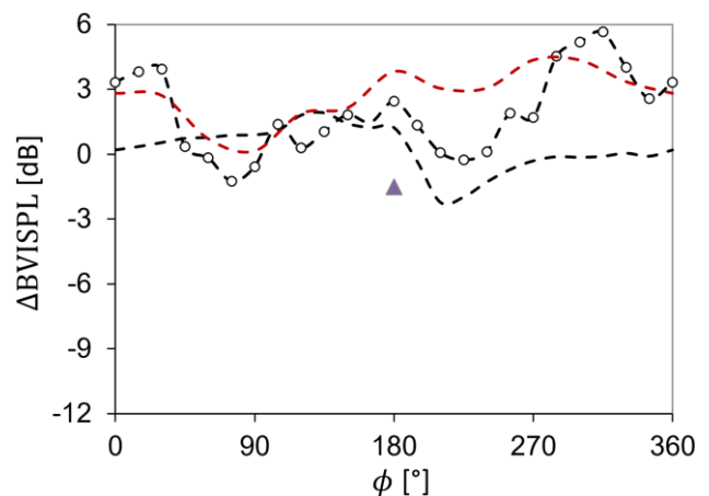
Figure 19: Change of noise level relative to its maximum as a function of 4p actuation with amplitudes of 50 % and 80 %. Dashed line with circles is the US 80 % amplitude result. Triangle symbols are results from DLR-S4
