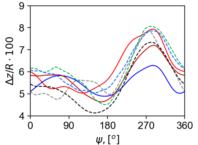
Figure 34: Vertical blade tip deflection, C_T/\sigma = 0.13
