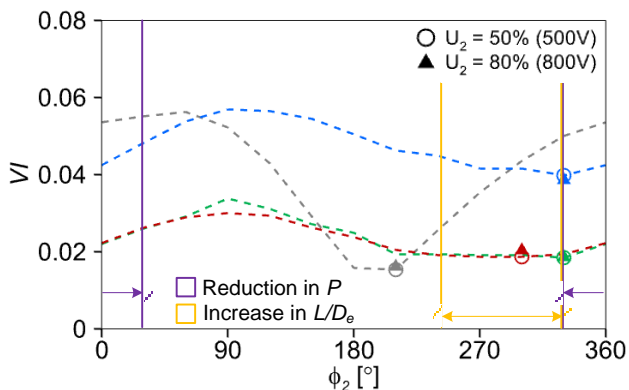
Figure 44: Effect of phase sweep on VI at dynamic 2p actuation ( U_0 = 400 V)
