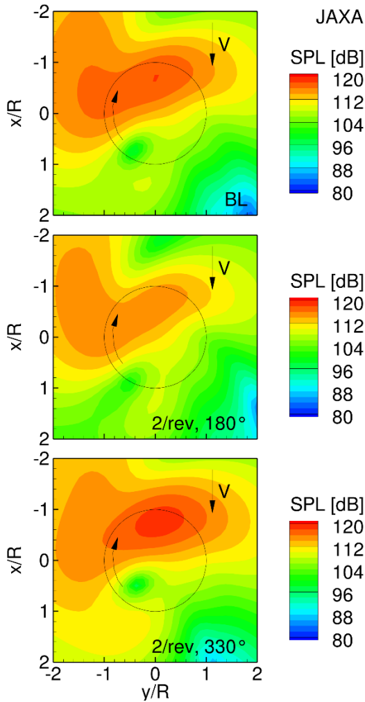
Figure 27: Noise level results of JAXA code in the horizontal plane 1.1R below the rotor hub for baseline (BL), minimum and maximum noise
