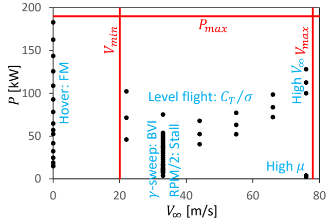
Figure 6: Power required for the test matrix conditions (DLR-S4)
