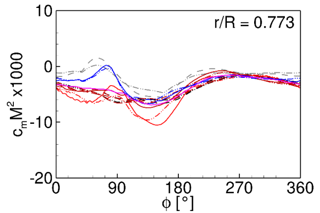
Figure 25: Sectional moment coefficient at 77.3 % R . Active twist results shown as dash-dot-dot
