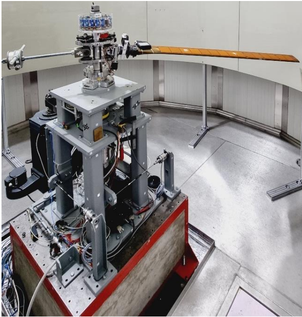
Figure 5: STAR blade in the whirl tower
