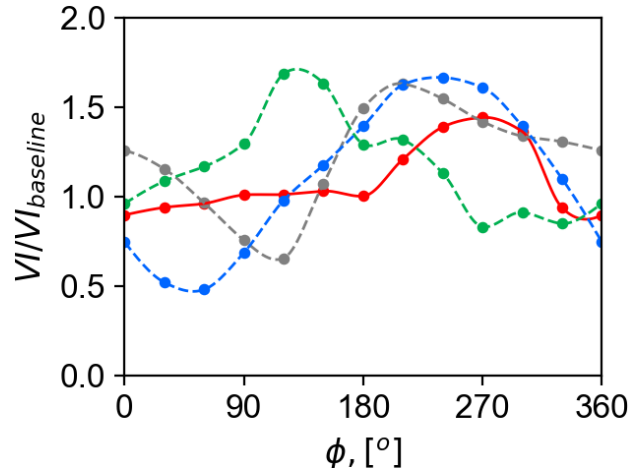
Figure 36: Vibration intrusion index, C_T/\sigma = 0.13 , 2p phase sweep
