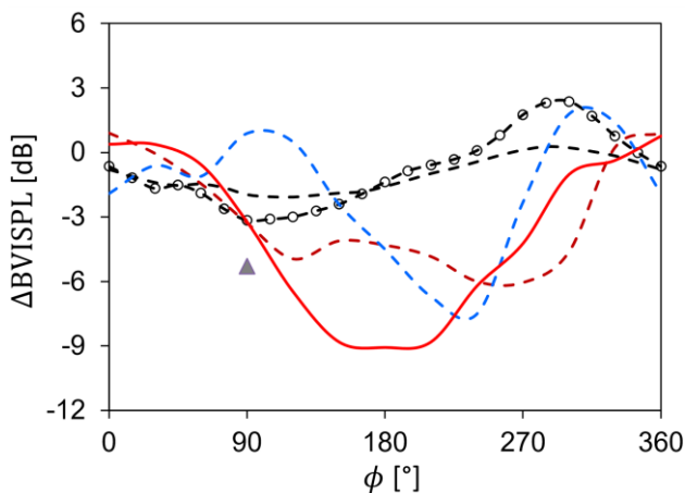
Figure 17: Change of noise level relative to its maximum as a function of 2p actuation with amplitudes of 50 % and 80 %. Dashed line with circles is the US 80 % amplitude result. Triangle symbol is the result from DLR-S4
