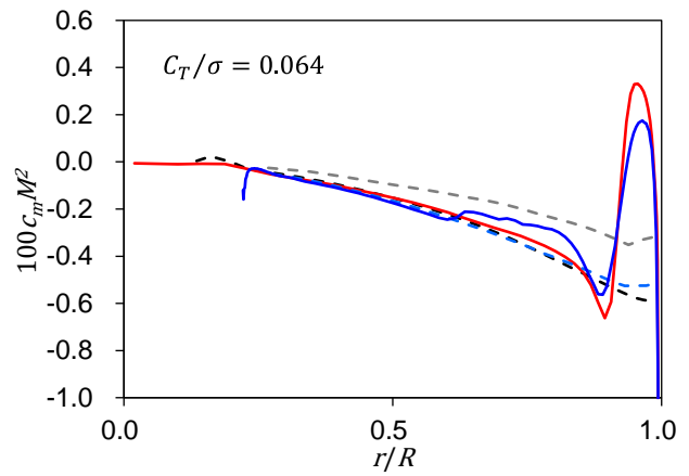
(a) Pitching moment coefficient for C_T/\sigma = 0.064
