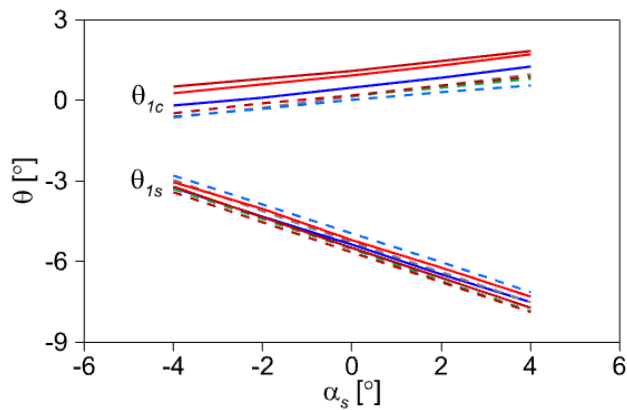
Figure 37: Comparison of trim control angles with shaft angle changes
