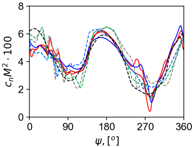
Figure 31: Section normal load coefficient, r/R = 0.67 , C_T/\sigma = 0.13
