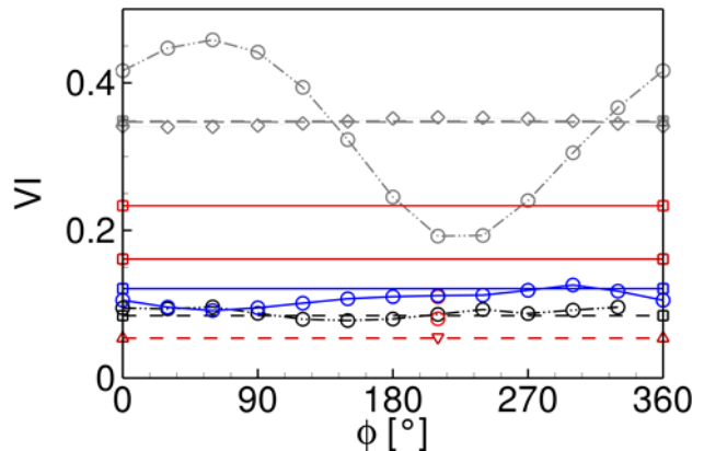
Figure 21: Vibration index results for baseline (horizontal line), 1p (DLR-S4 only) and 2p actuation
