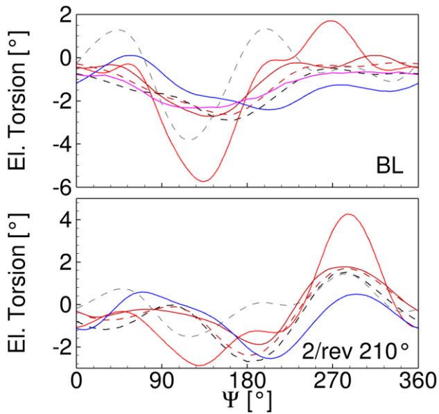
Figure 26: Tip elastic torsion prediction in the high-speed rotor case
