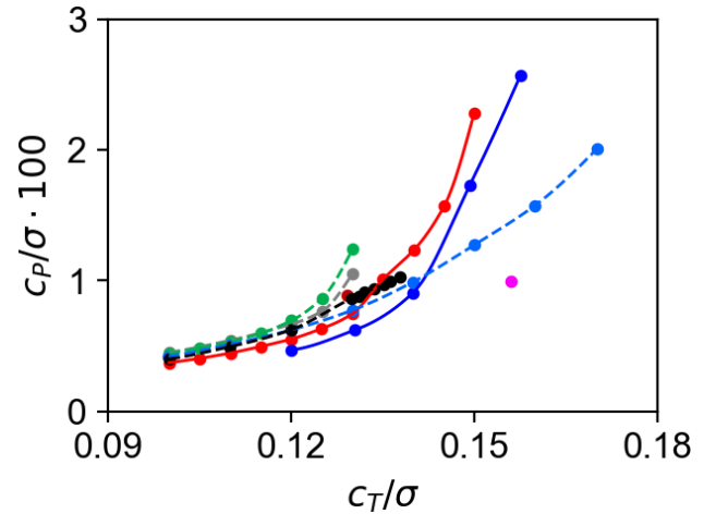
Figure 29: Power required, high load condition
