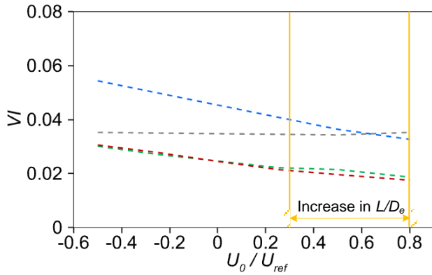
Figure 43: Effect of voltage sweep on VI at steady 0p actuation ( U_0 = 400 V)
