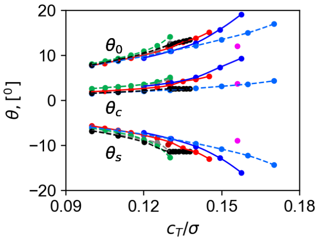
Figure 28: Control angles of the high load condition
