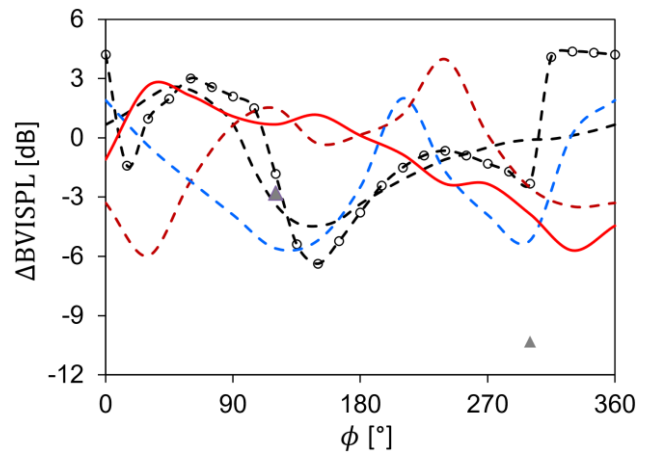
Figure 18: Change of noise level relative to its maximum as a function of 3p actuation with amplitudes of 50 % and 80 %. Dashed line with circles is the US 80 % amplitude result. Triangle symbol is the result from DLR-S4
