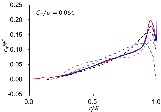
Figure 12: Radial distribution of sectional normal force for C_T/\sigma = 0.064
