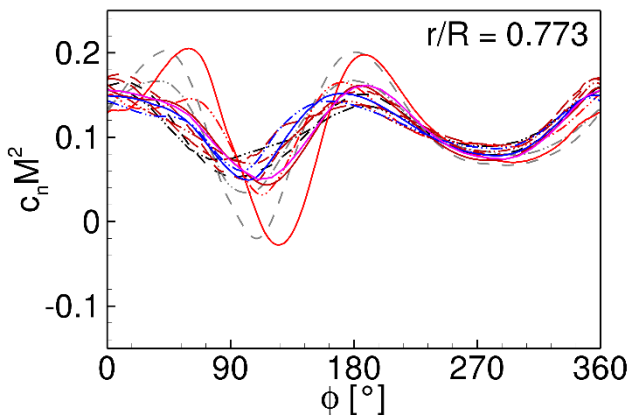
Figure 23: Normal force coefficient at 77.3 % R . Active twist results shown as dash-dot-dot
