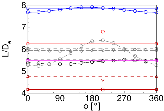
Figure 22: Lift to Drag-equivalent for baseline (horizontal lines), 1p (DLR-S4 only) and 2p actuation
