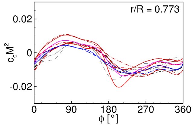
Figure 24: Chordwise force coefficient at 77.3% R . Active twist results shown as dash-dot-dot
