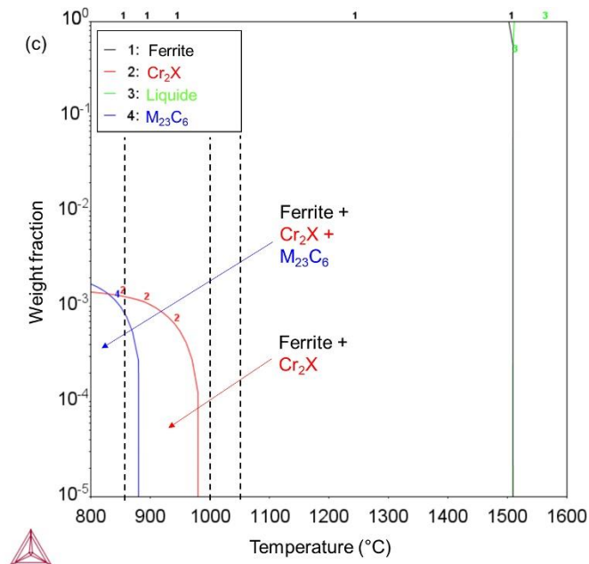
Figure 3: Phase diagrams for unstabilized grades, with “X” of Cr 2 X being mostly N, obtained with the TCFE10 base from Thermo-Calc software.
