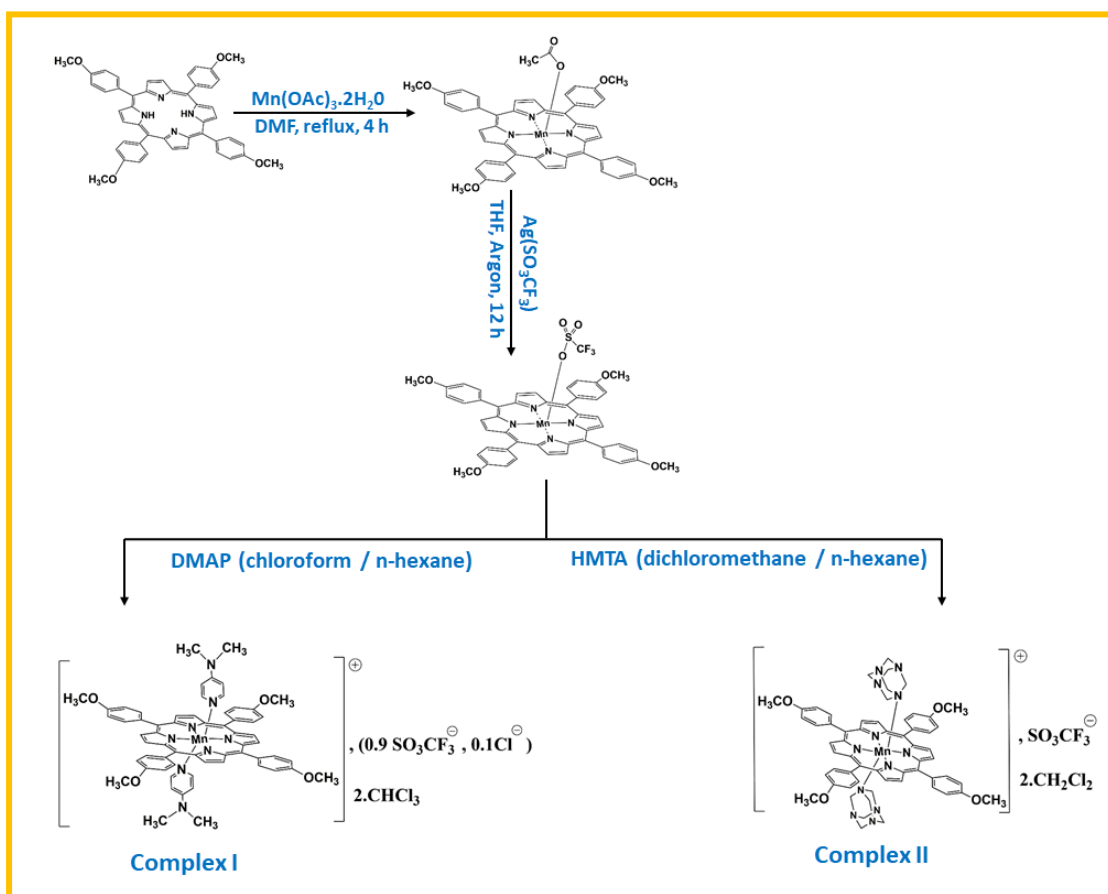
Scheme 1. Scheme of the synthesis of [\text{Mn}^{\text{III}}(\text{TMPP})(\text{DMAP})_2](0.9\text{SO}_3\text{CF}_3)(0.1\text{Cl}) \cdot 2\text{CHCl}_3 ( I ) and [\text{Mn}^{\text{III}}(\text{TMPP})(\text{HMTA})_2](\text{SO}_3\text{CF}_3) \cdot 2\text{CH}_2\text{Cl}_2 ( II ).
