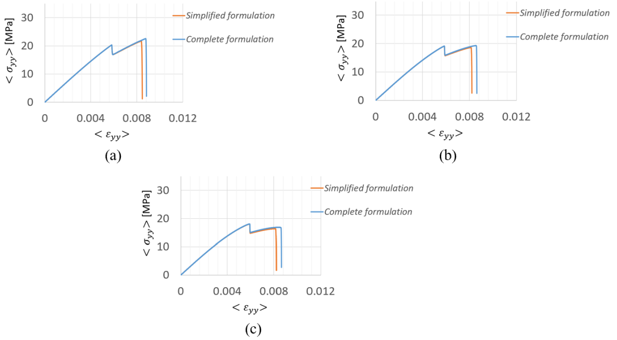
Figure 19: The macro-level \sigma - \epsilon relations for different l_c values and for the model with notch and fiber under tension: (a) l_c = 2.70 \times 10^{-4} mm; (b) l_c = 5.40 \times 10^{-4} mm; (c) l_c = 8.10 \times 10^{-4} mm.
