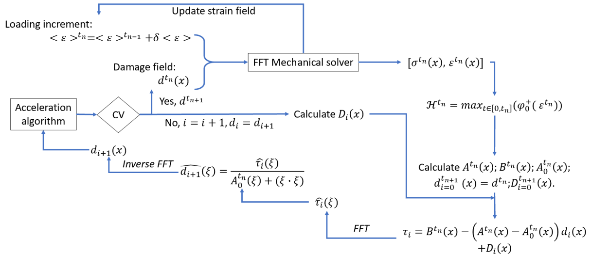
Figure 2: The flow chart of the implementation of the complete formulation into an FFT solver. CV means convergence check.
