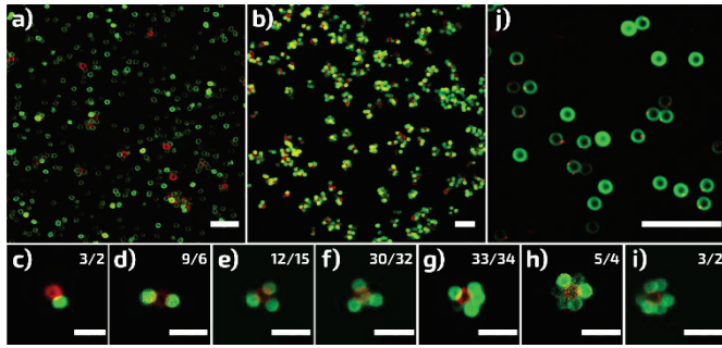
Fig. 2 Confocal fluorescence microscopy images of clusters obtained by incubating 1.6 \mu\text{m TPM}_A \sim \text{Ink}_{565} and 1.5 \mu\text{m PS}_B particles in a 1:40 ratio a) before and b) after purification. c-i) Zoom on the different clusters containing 1 to 7 PS particles. Their relative amounts (in %) in the sample before/after purification are given at the top right corner of each image. j) Confocal fluorescence microscopy image of the patchy PS particles resulting from the strand-displacement disassembly of \text{TPM}_A \sim \text{Ink}_{565} \sim \text{PS}_B clusters. Scale bar of 10 \mu\text{m} for a, b and j and 5 \mu\text{m} for c to i.
