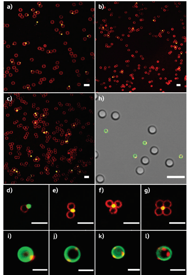
Fig. 3 Confocal fluorescence microscopy images of the clusters obtained by incubating \text{TPM}_B and \text{PS}_A \sim \text{Ink}_{565} in a 1:40 ratio followed by the addition of the Y^*_{488}\text{-B}^* passivation strand. The diameter of the TPM particles is: a) 1.1 \mu\text{m} ( \alpha = 4.39 ), b) and d-g) 1.6 \mu\text{m} ( \alpha = 3.02 ), c) 2 \mu\text{m} ( \alpha = 2.42 ). h) Confocal fluorescence microscopy images (Alexa488, green channel; Atto565, red channel) with transmission microscopy (grey channel) of \text{PS}_A \sim \text{Ink}_{565} \sim \text{TPM}_B & Y^*_{488}\text{-B}^* ( \alpha = 3.02 ) clusters after strand displacement reaction using \text{Eject}_X strand. i-l) Zoom on the patchy TPM particles with an increasing number of patches obtained after strand displacement reaction using \text{Eject}_X ( \alpha = 3.02 ). Scale bar of 10 \mu\text{m} for a to h and 2 \mu\text{m} for i to l.
