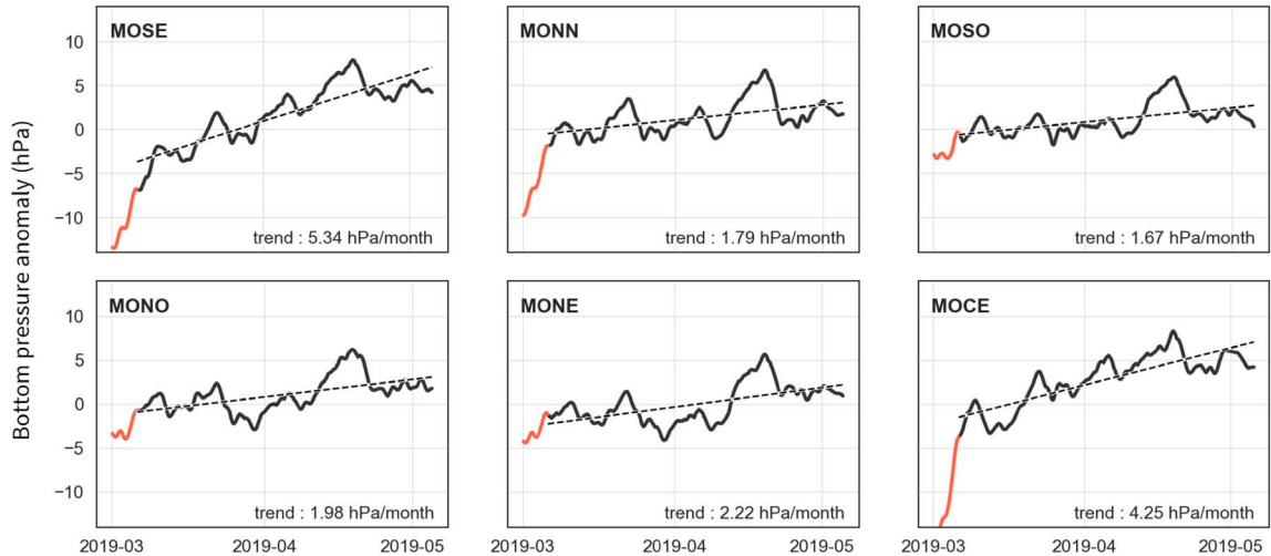
Figure 3. Bottom pressure anomalies (BPA) from six OBP records (February to May 2019), after applying the Demerliac filter and correcting the ocean signal contribution from the ECCO2 model. The first five days of data (red portions) are not used in trend estimates. Dashed lines represent the linear trend of each BPA series, for which the value is annotated on the bottom right corner.
