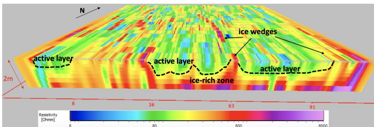
Figure 4 The shallow 3D resistivity grid (100 m X 100 m X 2 m) seen from the top: it images the active (conductive) layer and ice wedges (long resistive ridges) characteristic of Adventdalen permafrost.
