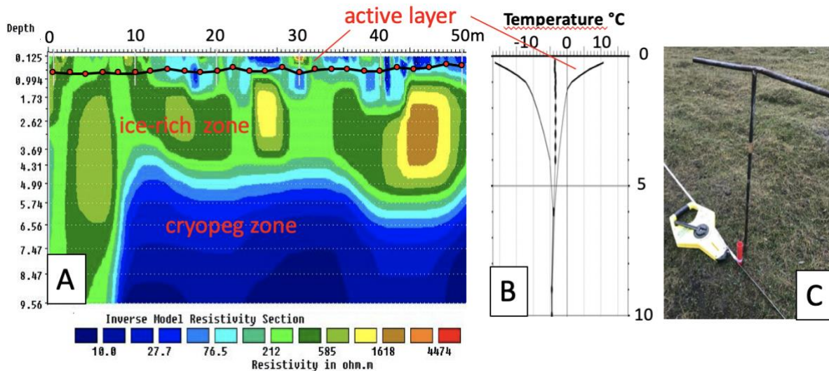
Figure 3 A) Vertical resistivity model with proposed soil interpretation in red. The depth of the frozen layer measured manually is marked as red symbols. B) Minimum and maximum ground temperature measured in A6 monitoring borehole: the ground temperature at 10 m depth is -5 \text{ }^\circ\text{C} . The symbols mark the annual average. C) Mechanic probe used to measure the depth of the thaw layer.
