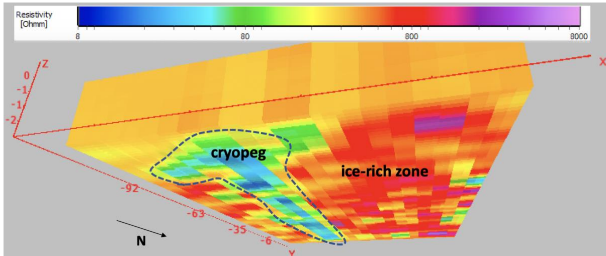
Figure 5 The deeper 3D resistivity grid (100 m X 100 m X 2.8 m) seen from below: it images the bottom of the ice-rich soil (in red) and reveals a conductive patch (in blue) which belongs to the cryopeg.
