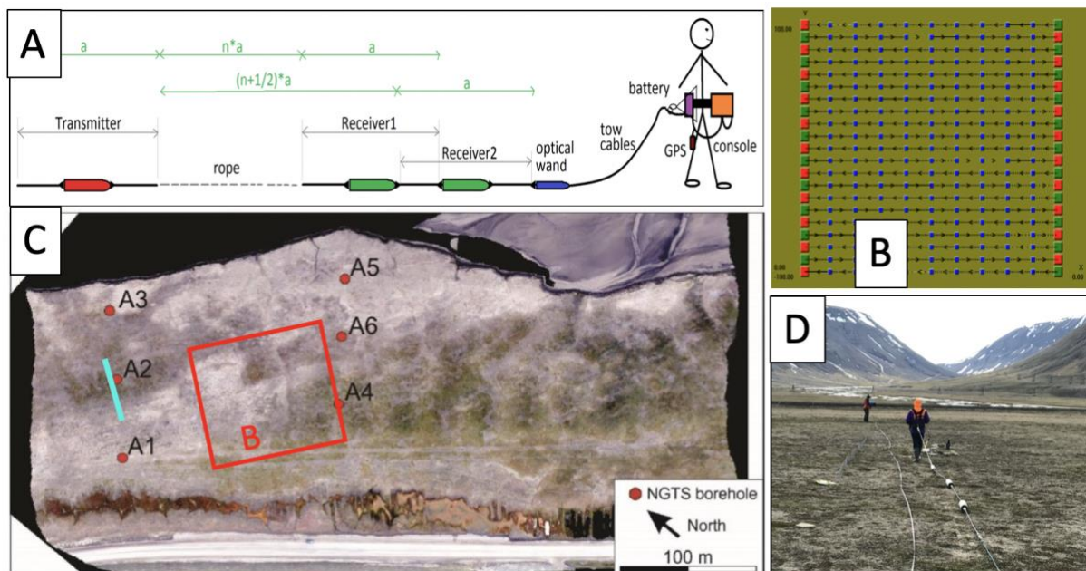
Figure 2 A) CCR acquisition with a streamer: different dipole sizes can be chosen by changing the rope length between the transmitter antenna and the two receivers. B) A map mode consists of towing the streamer along parallel lines. The survey consists of 21 lines separated by 5 m. C) Aerial image of the study site with the two types of acquisition: a 50 m long profile marked in blue and a 100 X 100 m box marked in red. A6 is a ground temperature monitoring borehole (Fig. 3B). D) Photo of the field survey.
