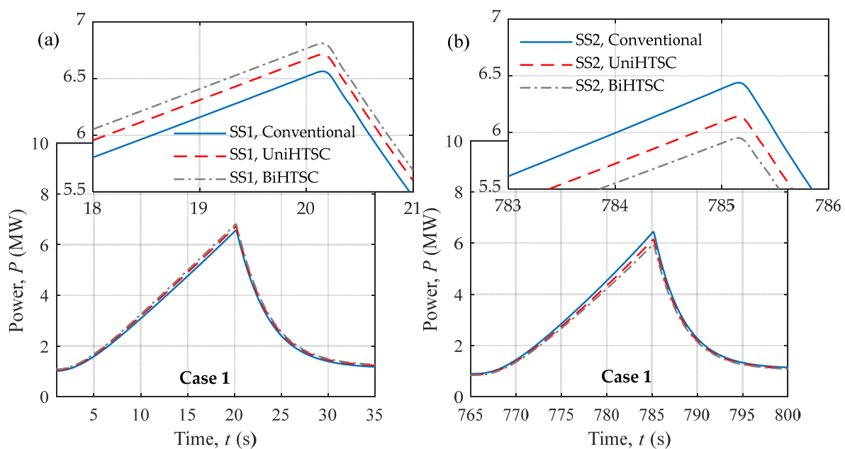
Figure 19. Peak instantaneous power supplied by the two substations for the three cable technologies in scenario 1: (a) SS1 at t = [0, 35] s, (b) SS2 at t = [765, 800] s.
