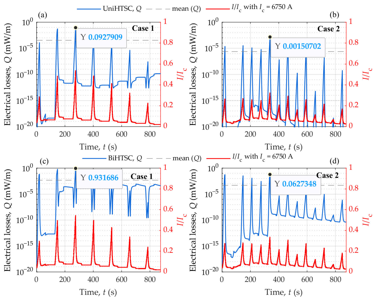
Figure 22. AC losses of the superconducting cable as a function of time; the second y -axis, on the right side of the figures, is the ratio I/I_c , with I_c being the critical cable current. (a,b) present the losses
