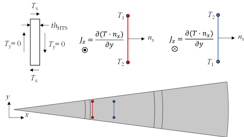
Figure 8. Boundary conditions for the T-formulation in the FEM.
