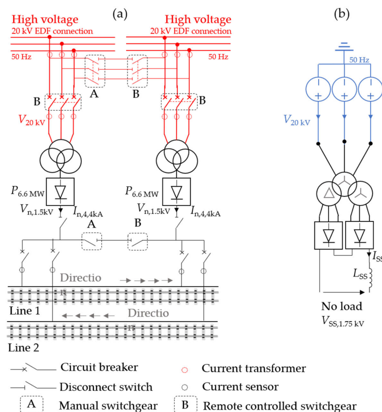
Figure 10. (a) Typical diagram of a 1.5 kV substation and the connection to the high voltage lines at 20 kV without showing the current return through the rails; (b) equivalent circuit of the substation implemented in Simulink. EDF is the acronym for Electricité De France.
