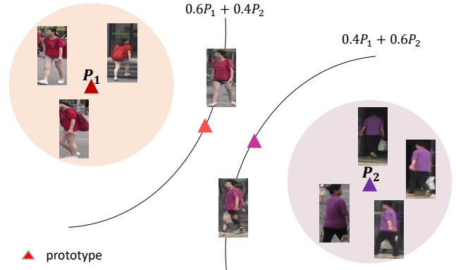
Fig. 4. Mixup Contrast targets at learning a smoother decision boundary between two persons P_1 and P_2 by contrasting in-between samples with in-between prototypes.
