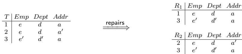
Fig. 1 An inconsistent table and its two repairs
