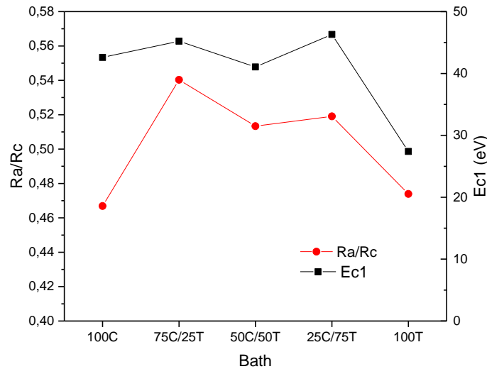
Fig. 10. Ratio Ra/Rc compared to E_{C1} for silver coatings with 100C, 75C/25T, 50C/50T, 25C/75T and 100T baths
