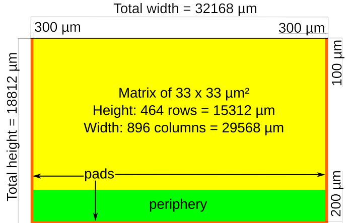
Figure 2: Design schematic for the OBELIX chip.
