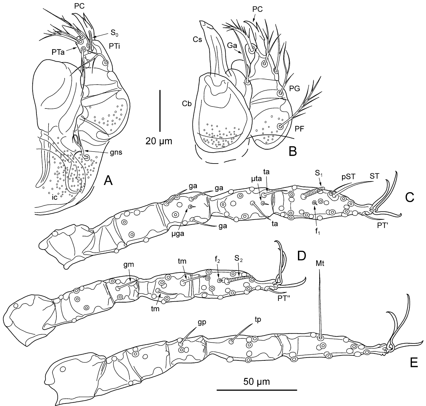
Figure 6 Microtrombicula abyssinica (Radford, 1947), additional specimen: A – ventral aspect of gnathosoma; B – dorsal aspect of gnathosoma; C – leg I (trochanter – tarsus); D – leg II (trochanter – tarsus); E – leg III (trochanter – tarsus). Abbreviations: Mt – mastitarsala. Other abbreviations as on Figure 3. Scale bars: A, B – 20 µm; C – E – 50 µm.
