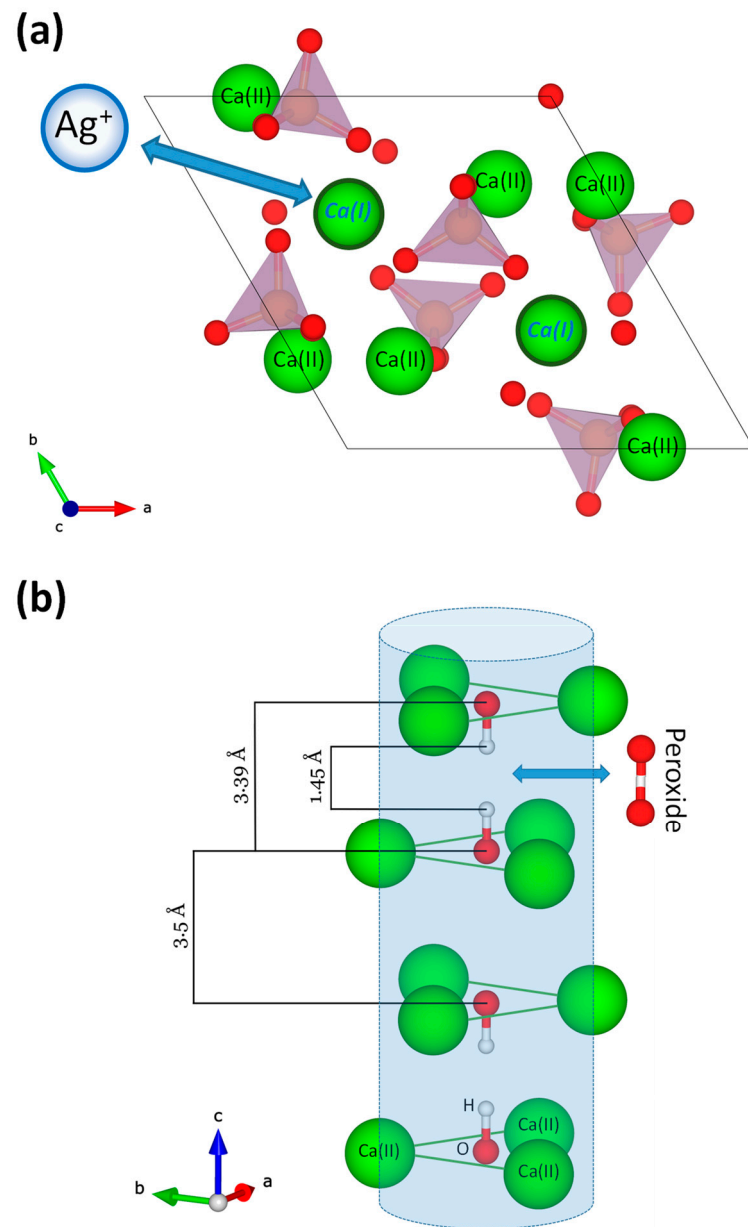
Figure 3. Structural arrangement of ions in the apatite structure. (a) Representation in the ab-plane showing cationic sites occupied by Ca^{2+} ions as Ca(I) and Ca(II) and the reported substitution of Ag^+ in Ca(I) sites; (b) apatitic channels parallel to the c-axis and formed by Ca(II) sites. Some specific distances involving the O and H atoms in OH^- ions are indicated. The peroxide ion O_2^{2-} is modeled considering the O–O bond length in H_2O_2 (close to 1.48 Å): 1 peroxide ion is hypothesized to replace two adjacent OH^- ions.
