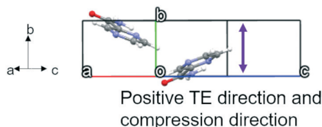
Fig. 5 Unit cell of form \gamma and the maximum thermal expansion and compression directions (purple arrow).
