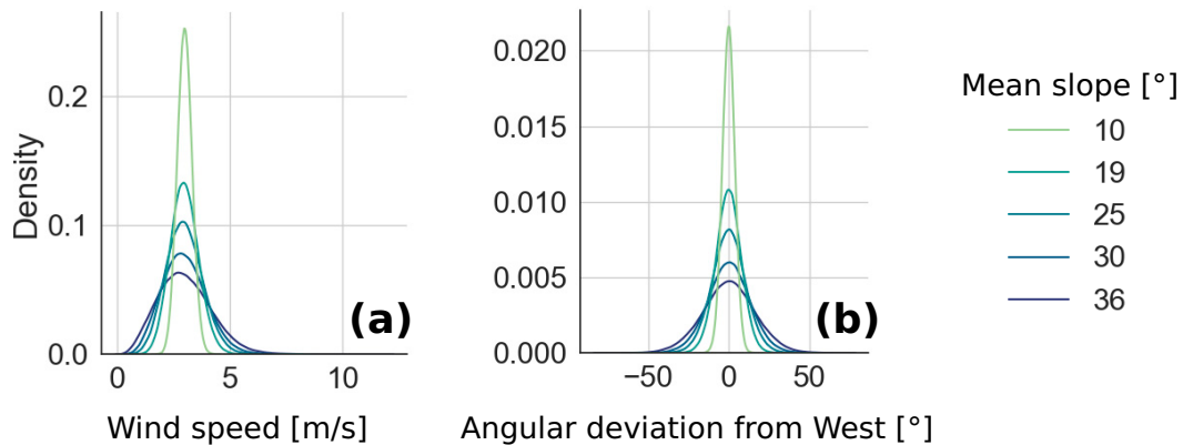
FIG. 2. (a) Wind speed and (b) angular deviation distributions as simulated by ARPS on the 7279 Gaussian topographies. Such winds constitute the training dataset used to fit the CNN of the DEVINE model.
