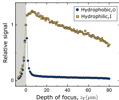
Figure 3. Sample data Relative intensity during a z -scan into a 70 wt.% glycerol solution of 4-DASPI (white area), from the hydrophobic glass (blue, showing a spike due to the adsorbed dye) or the hydrophilic glass (yellow, no adsorption detected).
