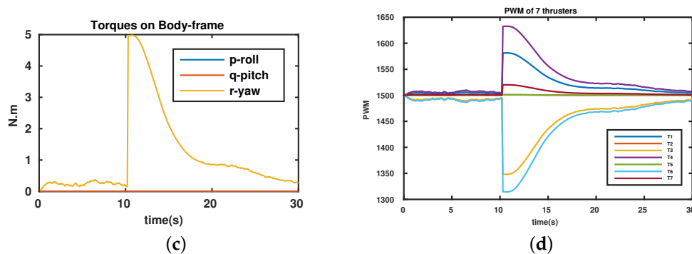
Figure 12. Yaw control of the UR. (a) Position and direction of thrusters of UR in the yaw control. (b) Yaw angles. (c) Applied torques. (d) PWM ( \mu\text{s} ) of thrusters.
