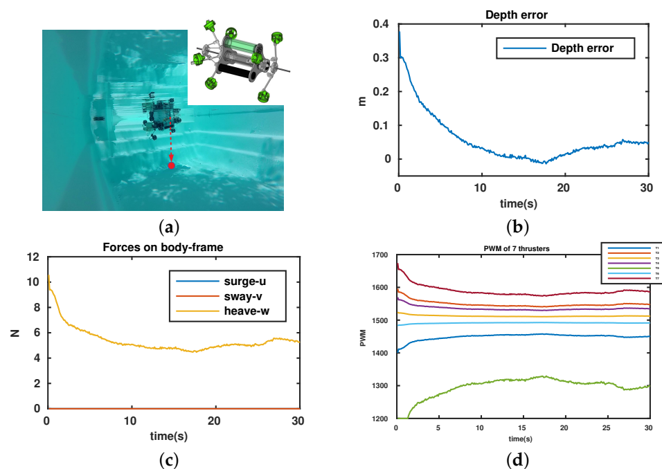
Figure 13. Depth control of the UR. (a) Mission description, position, and direction of thrusters in the depth control. (b) Depth error = desired depth–real depth. (c) Applied forces. (d) PWM ( \mu\text{s} ) of thrusters.
