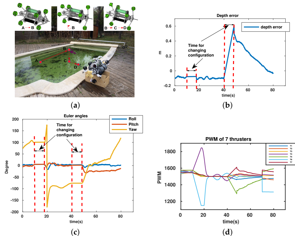
Figure 15. Integrated mission of Umbrella Robot. (a) Mission description, position, and direction of thrusters. (b) Depth error = desired depth–real depth. (c) Euler angles. (d) PWM ( \mu\text{s} ) of thrusters.
