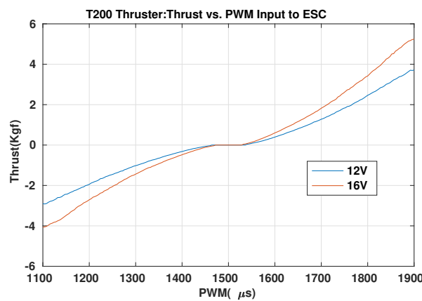
Figure 10. T200 thruster’s characteristics adapted from [32].
