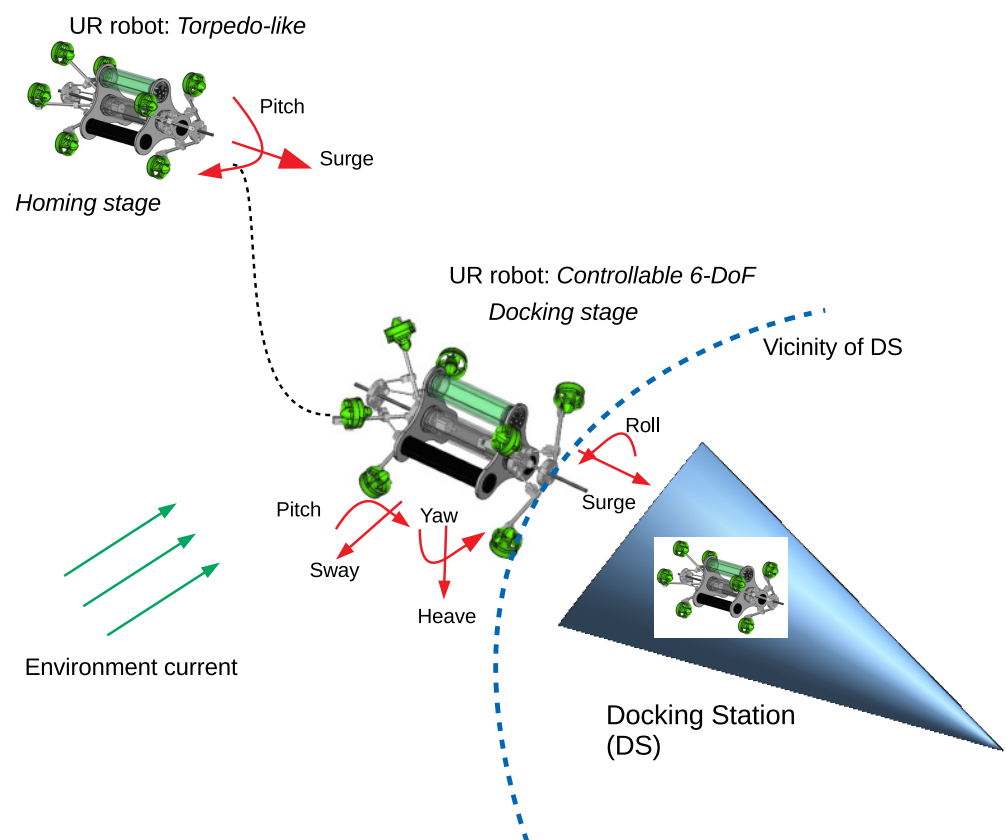
Figure 18. Concept of docking procedure of UR robot.
