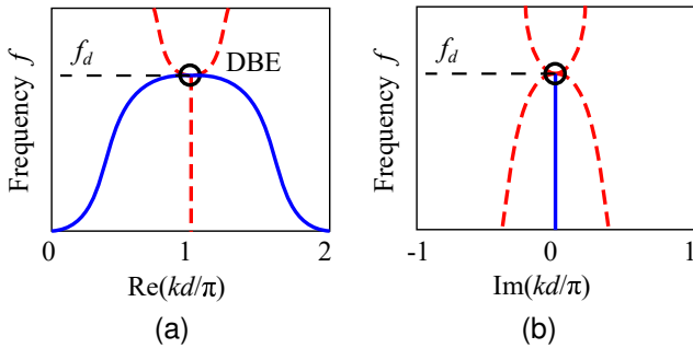
Fig. 1. Dispersion diagram of a periodic line of period d exhibiting a DBE. Propagating modes (blue lines), evanescent modes (red dashed lines). (a) Phase constant. (b) Attenuation constant.
