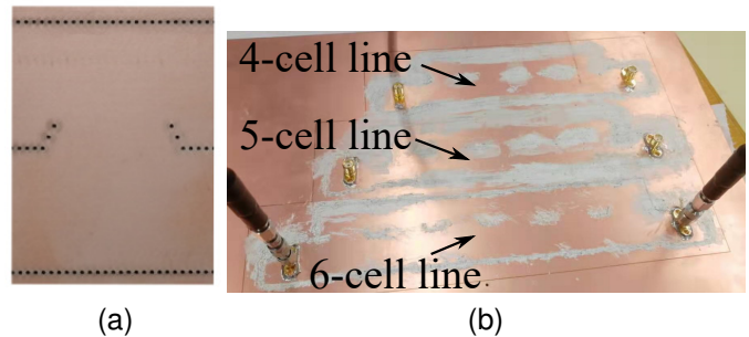
Fig. 19. Fabricated “low-loss corner-cell” SIWs lines. (a) Drilling details. (b) Final prototypes of 4-cell, 5-cell and 6-cell “low-loss corner-cell” SIWs lines. The white part is the metallic paste.
