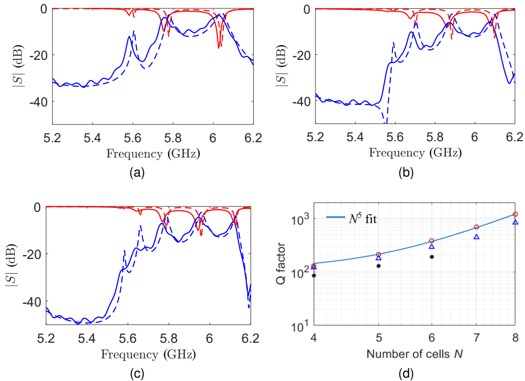
Fig. 20. Measurements of “low-loss corner-cell” SIW lines. (a) S parameters of 4-cell truncated line. Measurement results: solid lines . Simulation results: dashed lines . S_{11} : red lines . S_{21} : blue lines . (b) S parameters of 5-cell truncated line. (c) S parameters of 6-cell truncated line. (d) Loaded Q factor, computed with (3), versus the number of cells N . The resonance frequency f_{r,d} and the bandwidth BW are computed from the magnitude of S_{11} . Lossless lines without transition: ( red circles ), lossy lines with SMA-SIW transition: ( blue triangles ), experimental results ( black dots ).
