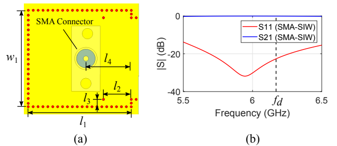
Fig. 17. The SMA-SIW transition.
