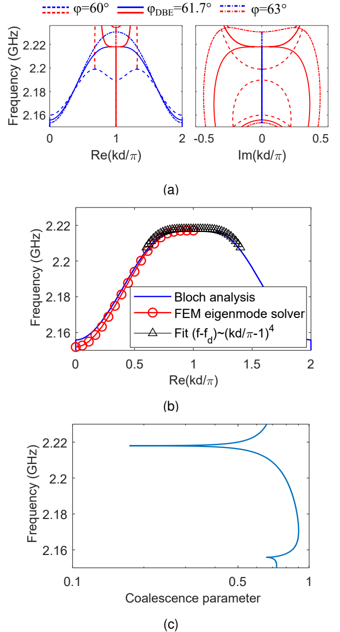
Fig. 3. Dispersion diagram of the lossless “double-coupler cell”. (a) Dispersion relations for different misalignment angles (propagating modes in blue curves, evanescent modes in red curves). (b) The dispersion diagram of the purely real -wavenumber mode when the DBE is achieved. (c) The level of the dip of the coalescence parameter reveals the closeness to an ideal DBE condition.
