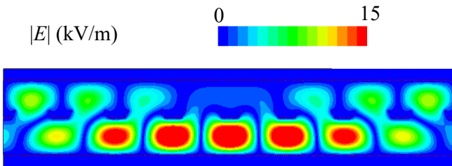
Fig. 15. The E -field distribution of 8-cell truncated SIWs of "low-loss corner-cell".
