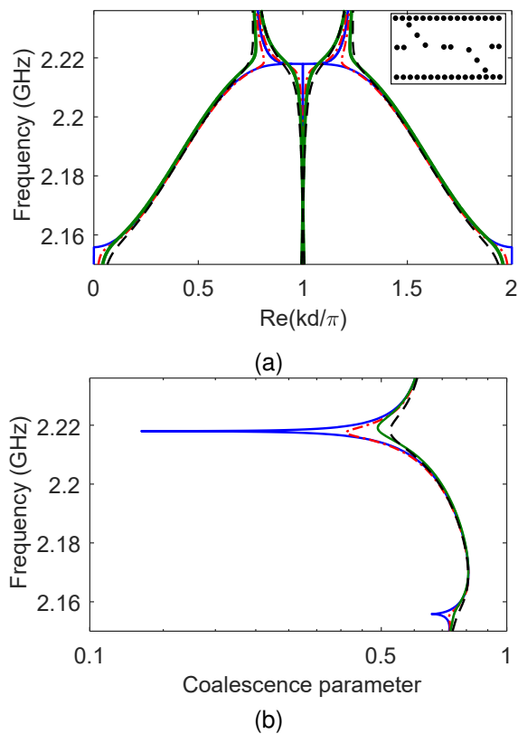
Fig. 4. Losses influence on DBE of “double-coupler cell” design. Four different cases are considered: lossless ( blue line ), only conductor losses ( red dashed line ), only dielectric losses ( green line ), and both conductor and dielectric losses ( black dashed line ). (a) Dispersion diagram. (b) Coalescence parameter.
