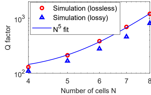
Fig. 16. Q -factor of "low-loss corner-cell" SIWs lines. Both lossless (red-circle mark) and lossy (blue-triangle mark) situations are considered. (a) The scaling of Q factor fits a N^5 law.
