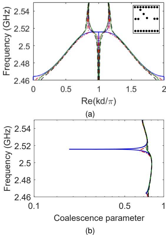
Fig. 7. Dispersion diagram of "single-coupler cell". The DBE is located at 2.516 GHz. Lossless (blue line), only conductor losses (red dashed line), only dielectric losses (green line), and both conductor and dielectric losses (black dashed line). (a) Dispersion diagram. (b) Coalescence parameter.
