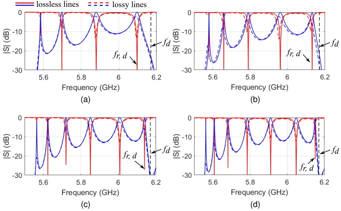
Fig. 13. S parameters of lossy truncated SIWs lines. S_{11} (red lines), S_{21} (blue lines). (a) 5-cell, (b) 6-cell, (c) 7-cell, (d) 8-cell.
