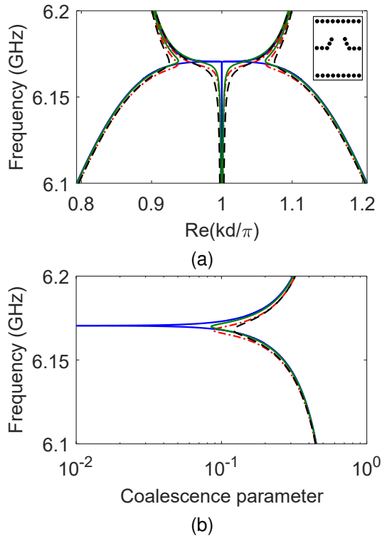
Fig. 12. The dispersion diagram of “low-loss corner-cell” design. The DBE frequency is at 6.17 GHz. Lossless (blue line), only conductor losses (red dashed line), only dielectric losses (green line), and both conductor and dielectric losses (black dashed line). (a) Dispersion diagram. (b) Coalescence parameter.
