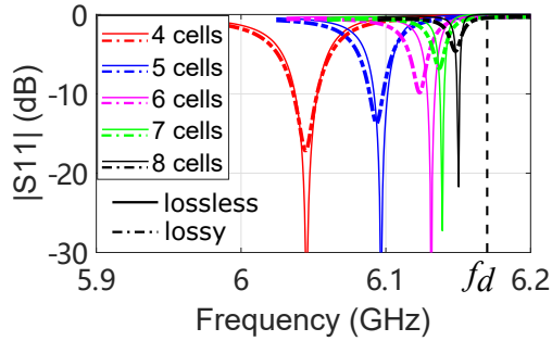
Fig. 14. Magnitude of S_{11} for different length "low-loss corner-cell" SIWs structures.
