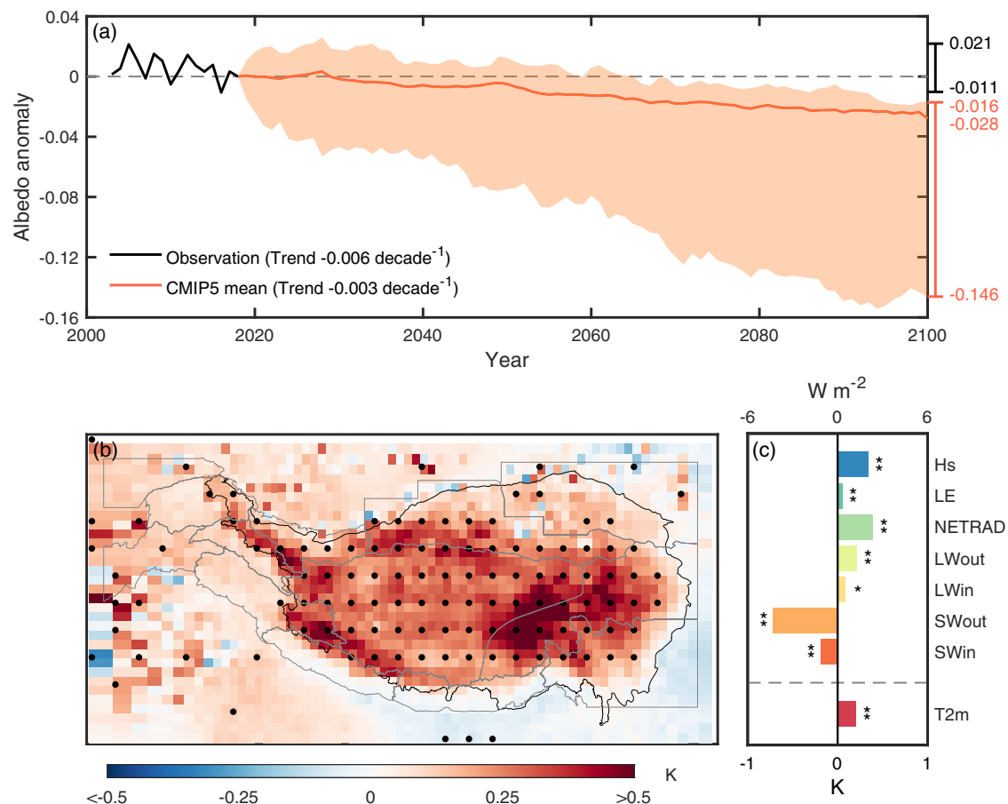
Fig. 1 | Changes of albedo and albedo-induced local climate in the Tibetan Plateau (TP). a Time series of albedo anomaly in the TP. The thick solid black line represents the albedo anomaly of observation during 2003–2018 CE, which is the annual mean albedo derived from the MODIS MCD43 product relative to its benchmark-year (2018 CE) value. The thick solid orange line and shaded orange area, respectively, represent the weighted average and ranges of future (2018–2100 CE) projection albedo anomaly derived from 35 global climate models (GCMs) in CMIP5. The future projection albedo anomaly derived from each CMIP5 GCM is the 5-year moving average of the annual mean albedo in RCP8.5 relative to its benchmark-year (2018 CE) value. Trends of the thick solid black and orange lines are about -0.006 \text{ decade}^{-1} ( p = 0.19 , Mann-Kendall test) and about -0.003 \text{ decade}^{-1} ( p < 0.01 , Mann-Kendall test), respectively. b The spatial pattern of the
