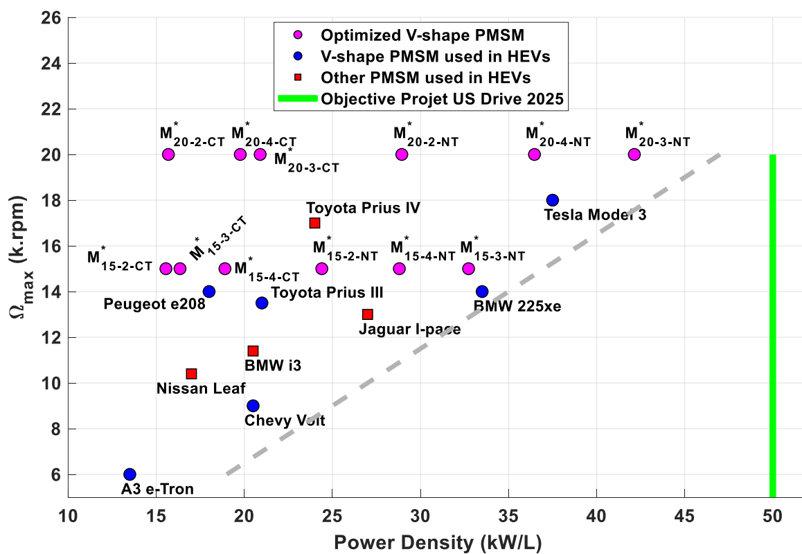
Figure 17. Maximum rotational speed vs. power density for optimal machines and other machines used in hybrid electric vehicles (HEV).
