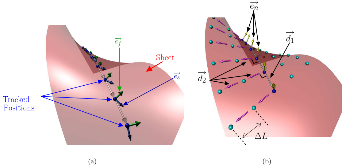
Figure 6: Steps used for the construction of the sheet. Figure (a) shows the reconstruction in the radial direction. At each position (blue spheres), the fiber direction \mathbf{e}_f and the sheet direction \mathbf{e}_s are determined from the data. The projected desired radial directions \mathbf{d}_1 are in transparent white. Figure (b) shows the reconstruction in the circumferential direction. The yellow vectors \mathbf{e}_n are the normals to the surface and the perpendicular directions \mathbf{d}_2 (shown in magenta) are the reconstructed circumferential directions.
