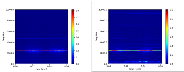
FIGURE 12. Artificial intelligence for acoustic data processing: visual comparison of spectrograms of a working engine (left: faulty conditions; right: healthy conditions)
