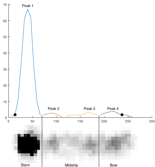
FIGURE 8. OSIRIS-FO: Scattering profile of a bulk carrier ship as estimated by the new feature extractor.
