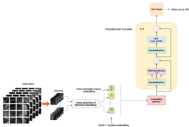
FIGURE 10. 3D vision transformers architecture used to predict prostate cancer aggressiveness.
