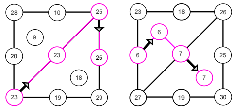
Figure 6 Left: A Morse stack F on a complex X , with, in pink, a \nabla_1 -path. Right: A Morse stack G on a complex X' , with, in pink, a \nabla_2 -path.
