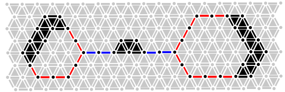
Figure 4 A simplicial stack F with two values (0 in gray and 1 in black, red, and blue) on a subset of a normal 2-pseudomanifold. In blue and red, the separating faces. In red, the biconnected faces.
