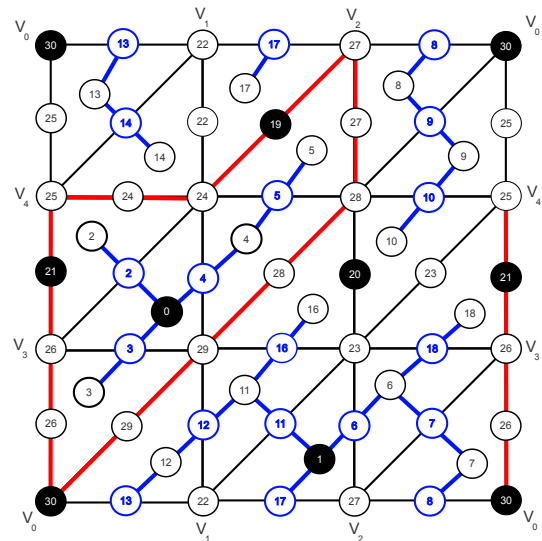
Figure 8 The Morse watershed (in red) on a Morse stack F defined on a 2D-torus. In blue, the watershed forest, which is the minimum spanning forest for \min(F) .
