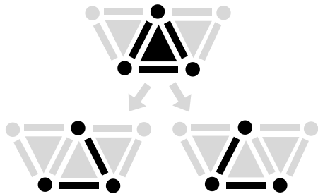
Figure 1 A simplicial stack F with two values (0 in gray, and 1 in black) on a complex X , and two different elementary collapses of F .
