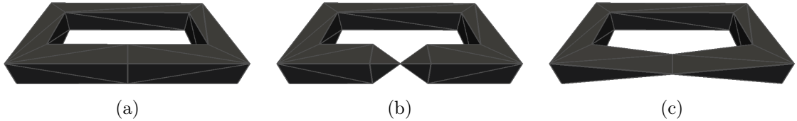
Figure 2 (a): A normal pseudomanifold, which is a torus, (b): A pseudomanifold, which is a pinched torus, and where the pinch face is a vertex, (c): A pinched torus where the pinch face is a segment. This is not a pseudomanifold.
