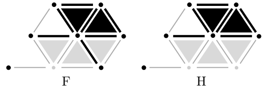
Figure 3 Two stacks F and H with two levels: altitude 0 (faces in light gray) and altitude 1 (faces in black). The stack H is an elementary collapse of F (at altitude 1). But F has three minima whereas H has only two. Thus, \min(H) is not an extension of \min(F) .
