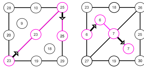
Figure 6 Left: A Morse stack F on a complex X , with, in pink, a \nabla_1 -path. Right: A Morse stack G on a complex X' , with, in pink, a \nabla_2 -path.
