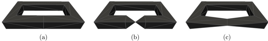
Fig. 1 (a): A normal pseudomanifold, which is a torus, (b): A pseudomanifold, which is a pinched torus, and where the pinch face is a vertex, (c): A pinched torus where the pinch face is a segment. This is not a pseudomanifold.
