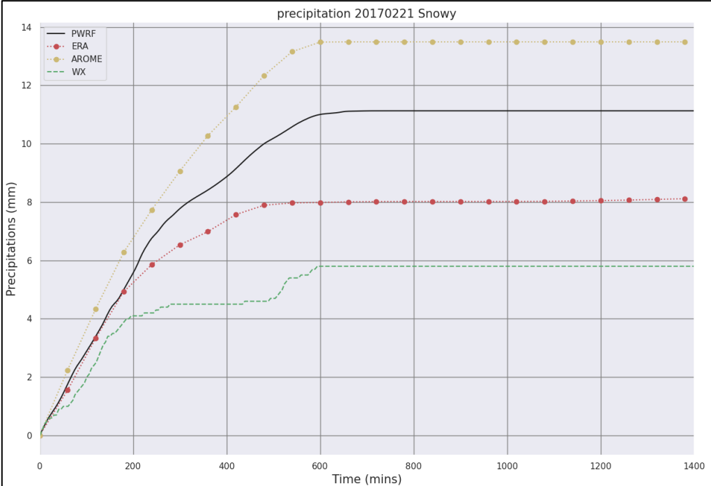
Figure 5 : Cumulative precipitation amount (water equivalent) on the SvalSat station on 02/21/2017, from PWRF simulations and from the various reference meteorological databases.
