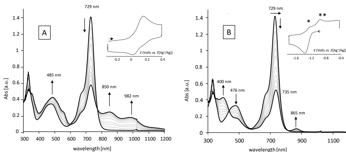
Figure 10: UV-vis spectra recorded during the oxidation (A) and reduction (B) of azaGaDIPY-OMe in DMF (0.1M TBAP) at a platinum gauze working electrode ( l = 0.5 mm, v = 10 mV/s). The current potential curves recorded at the working electrode are shown as insets.
