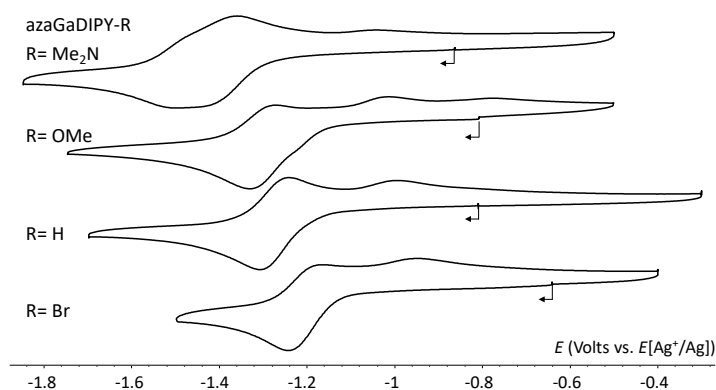
Figure 8: Voltammetric curves of DMF (0.1M TBAP) solutions of azaGaDIPY-R with R = \text{Me}_2\text{N} , \text{OMe} , \text{H} and \text{Br} ( \nu = 0.1 \text{ V s}^{-1} , \text{VC} \Phi = 3 \text{ mm} , E (volt) vs E_{\text{ref}}[\text{Ag}^+(10^{-2} \text{ M})/\text{Ag}] ).
