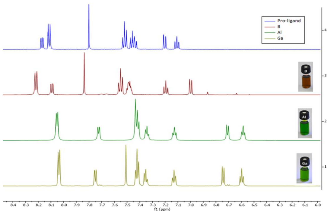
Figure 2: ^1\text{H-NMR} spectra of 3 , azaBODIPY-H , azaAlDIPY-H , and azaGaDIPY-H in \text{DMSO-d}_6 at 298 K.
