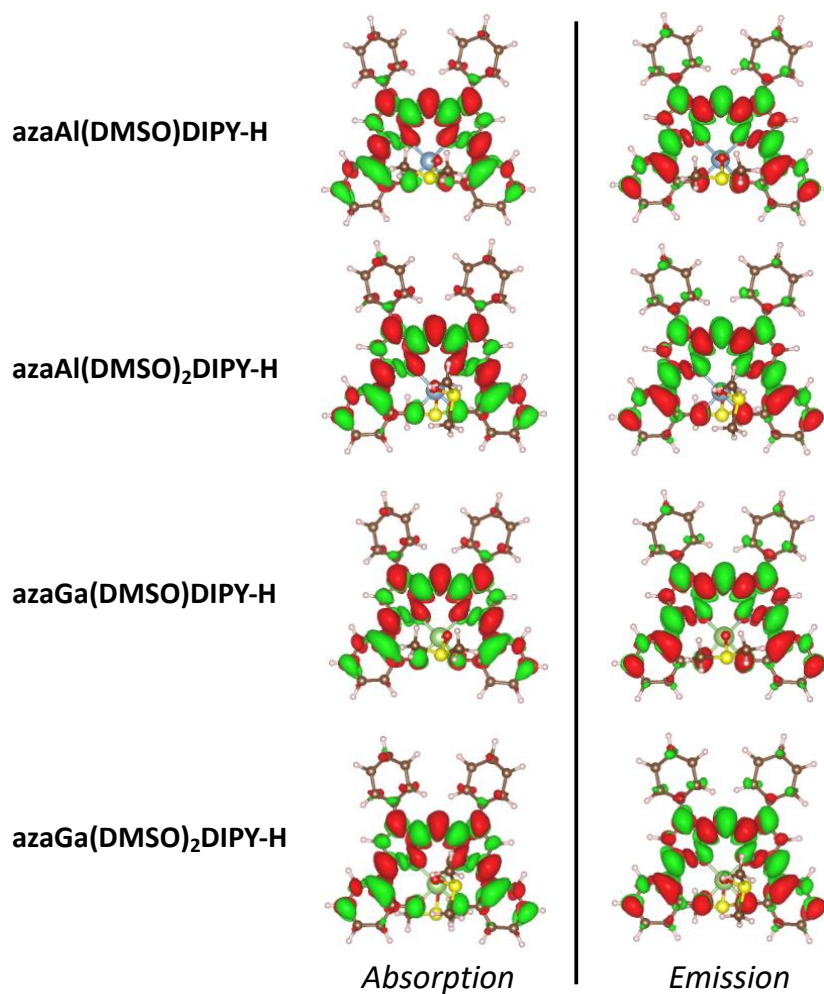
Figure 6: Density difference between the ground and excited state for absorption (left) and emission (right) (isovalue of 0.0005 au) for azaAl(DMSO) n DIPY-H and azaGa(DMSO) n DIPY-H compounds ( n =1, 2) in DMSO. Red and green surfaces represent respectively a gain and a loss of electronic density.
