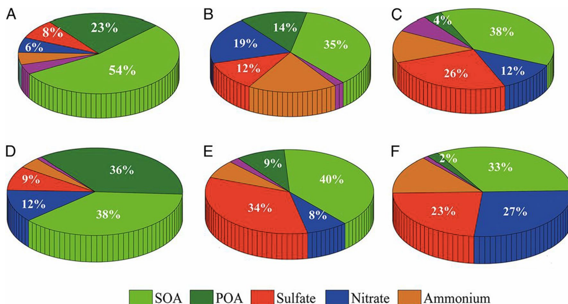
Fig. 3 Particle chemical compositions during the clean, transition, and polluted periods for the 25–29 September and 2–7 October episodes. SOA, secondary organic aerosol; POA, primary organic aerosols. (A–C) Chemical compositions for 80-nm (A), 100-nm (B), and 240-nm (C) particles were measured by the aerosol mass spectrometer at 1500 h on 25 September, 1200 h on 27 September, and 1800 h on 28 September, respectively. The three particle sizes (i.e., close to the mean size) are selected to represent the dominant features in the chemical composition during the clean, transition, and polluted peri-
