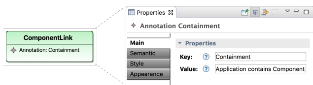
Fig. 8 Annotation mechanism.
