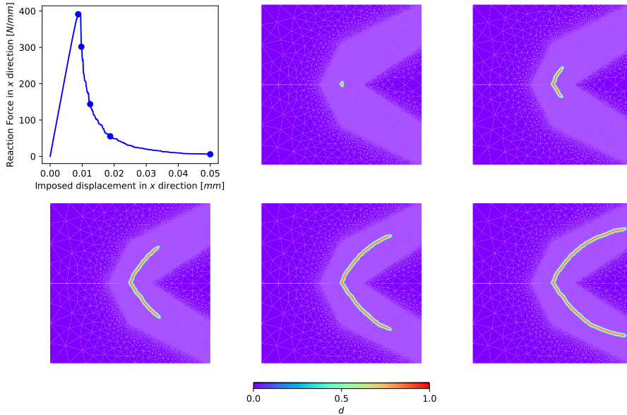
Figure 8: Shear test: symmetric traction/compression. Top left: load displacement curve. From left to right and top to bottom, damage field at the corresponding dot on the curve.
