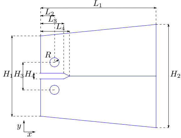
Figure 5: TDCB geometry definition.
