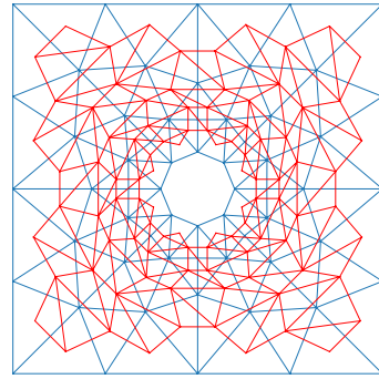
Figure 2: The finite element mesh (blue) and the Lip-mesh (red) built from the centroids of the blue mesh elements.
