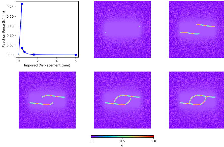
Figure 11: Two edge cracks, top left: load displacement curve. From left to right, damage field at the corresponding dot on the curve.
