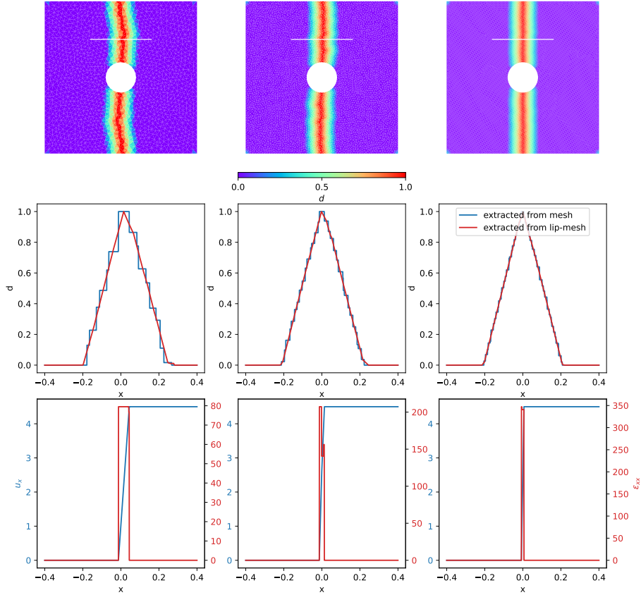
Figure 4: Convergence analysis: top damage field, below u_x , \epsilon_{xx} extracted from the white line for different meshes, at the end of the simulation.
