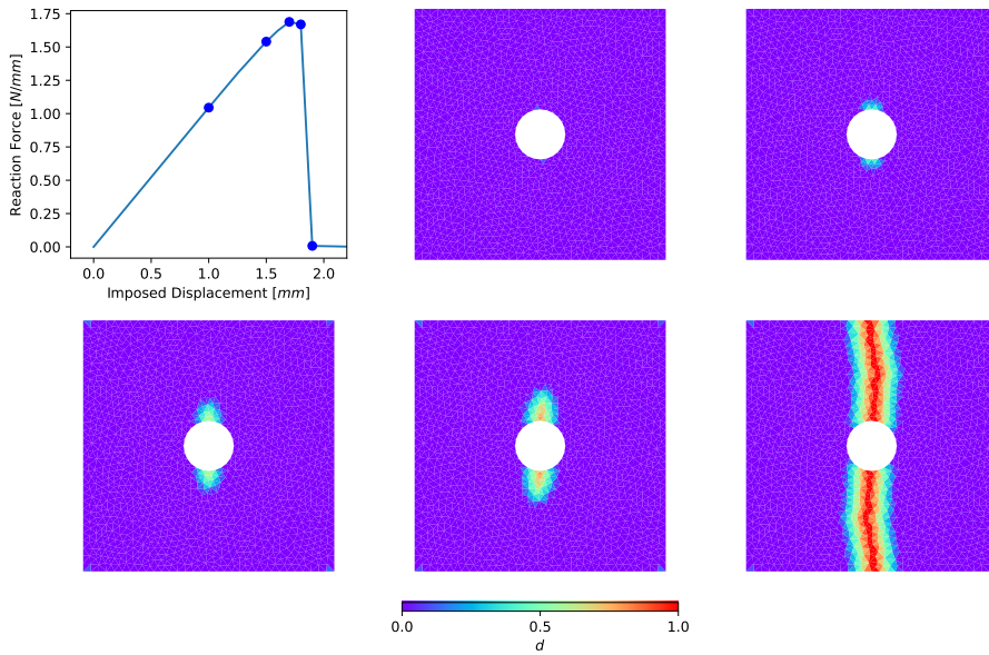
Figure 3: Load displacement curve and damage field for mesh 1.
