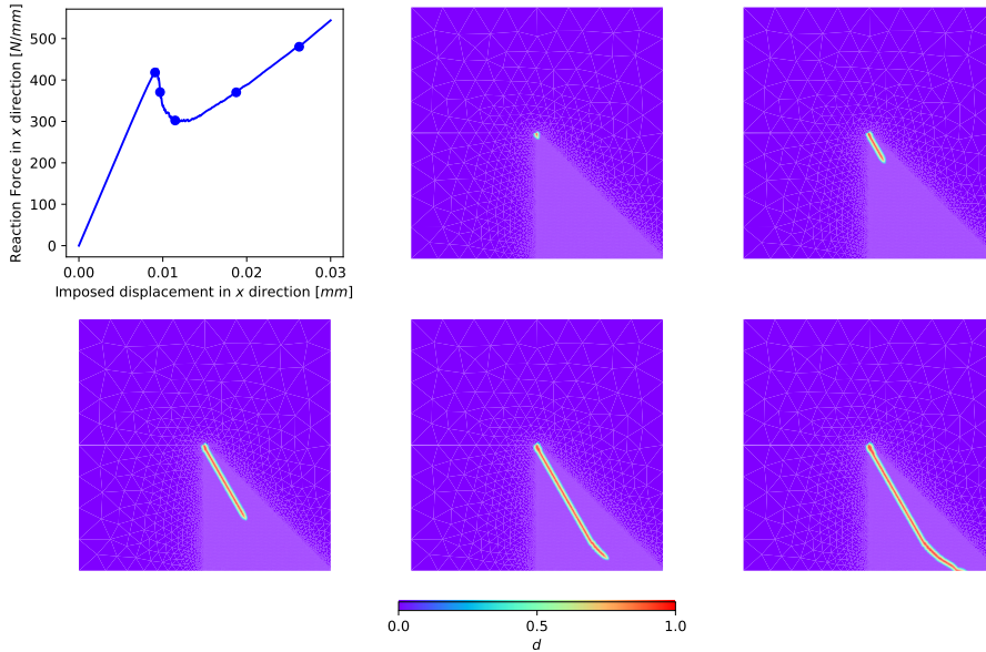
Figure 9: Shear test: Asymmetric traction/compression. Top left: load displacement curve. From left to right, top to bottom damage field at the corresponding dot on the curve.
