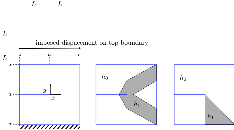
Figure 7: From left to right : shear test geometry and boundary conditions definition, mesh parameter for the symmetric case and the asymmetric case
