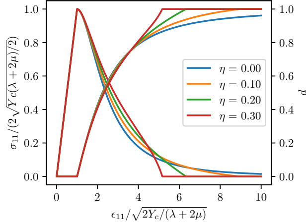
Figure 1: Influence of the \eta parameter on the stress/strain curve (left curves) and on the damage evolution with respect to strain (right curves).
