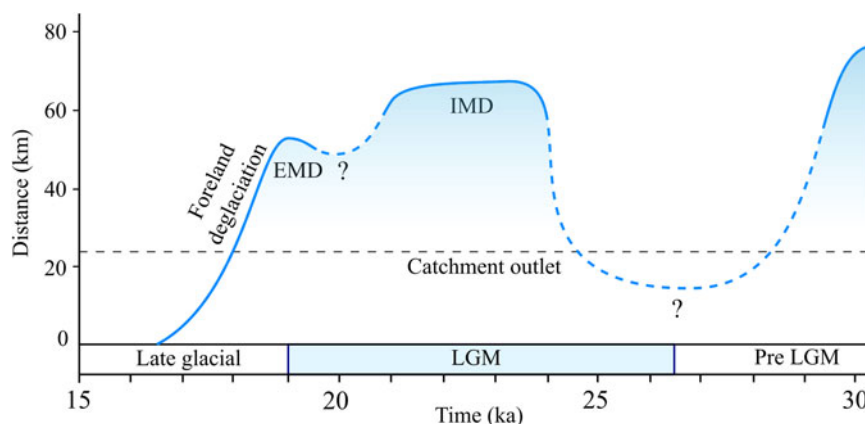
Figure 5. Time- distance diagram for the last glacial cycle glacier advances and retreat of the Lyonnais ice lobe based on OSL, ^{14}\text{C} , and our exposure ages. IMD = Intermediate Morainic Domain; EMD = Eastern Morainic Domain. Distance origin is located at the level of CUL 19-01 boulder.
