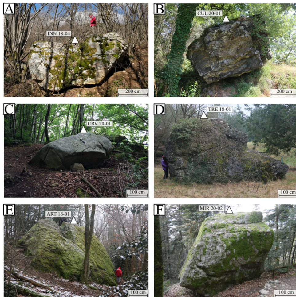
Figure 2. Examples of sampled boulders on the southern Jura: INN 18-04 (A); Rhône Valley: CUL 20-01 (B) and CRV 20-01 (C); Crémieu plateau: TRE 18-01 (D); Southwestern foreland: ART 18-01 (E); and Terres Froides: MIR 20-02 (F).
