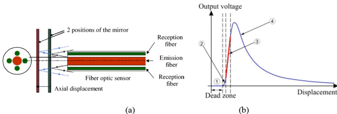
Fig. 2 The optical fiber displacement sensor
