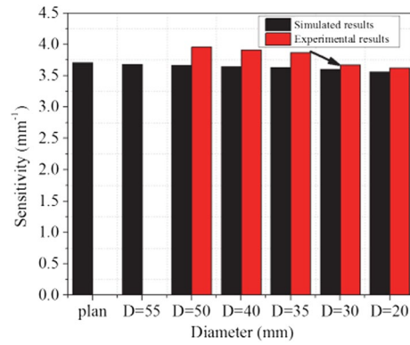
Fig. 10 Influence of the diameter of the reflective convex surface on the sensor sensitivity [22]
