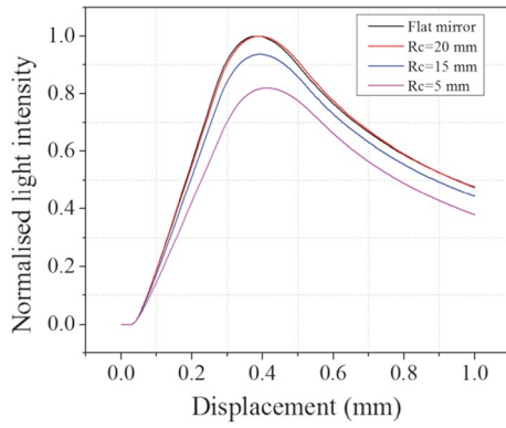
Fig. 8 Response curve for several radii of curvature [21]
