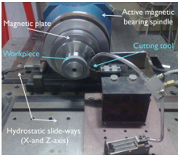
Fig. 12 Focus on the high precision lathe used in this study [22]
