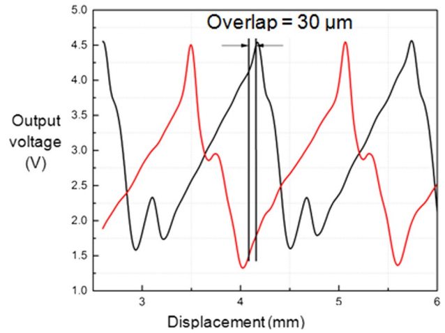
Fig. 19 Measurement of the grating displacement (mm)
