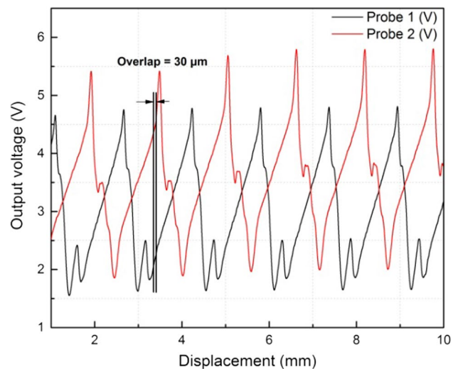
Fig. 23 Signals obtained at ( V_t=0.05 mm/s and V_r=20 rev./s)
