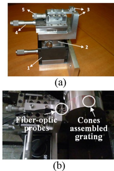
Fig. 17 Experimental set-up
