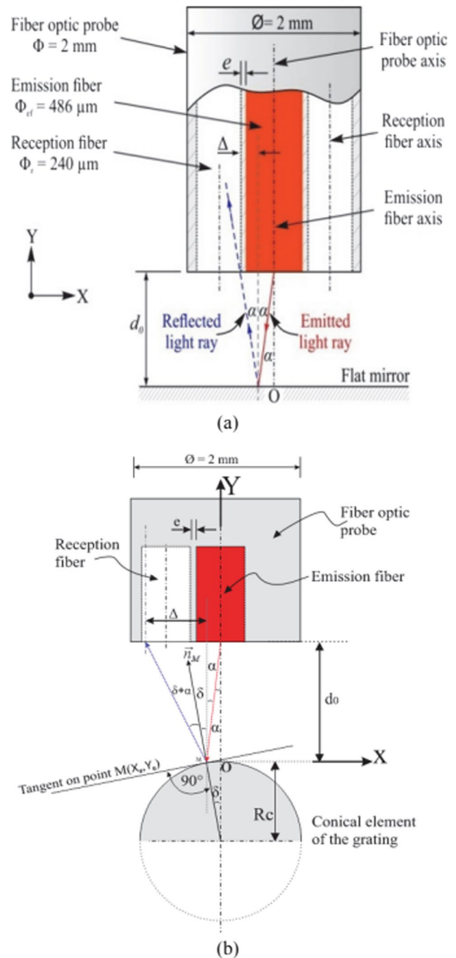
Fig. 7 Schematic diagram of the reflected light model a flat mirror, b convex mirror [22]
