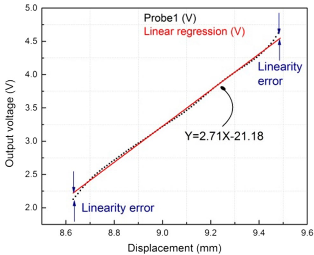
Fig. 21 Signal obtained on the sixth conical step
