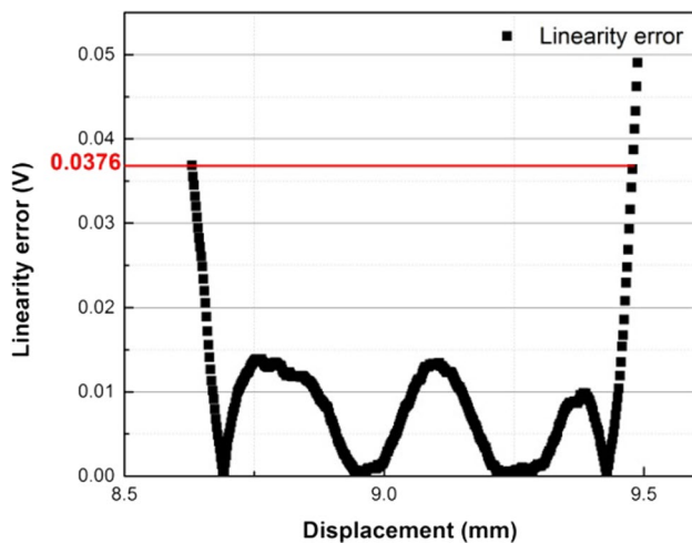
Fig. 22 Linearity error as a function of displacement
