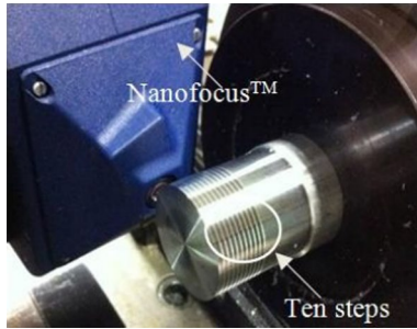
Fig. 14 Geometric characteristics
