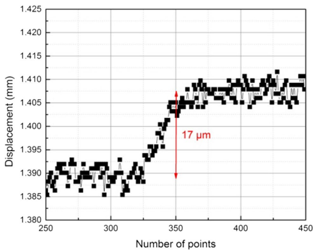
Fig. 24 Resolution measurement
