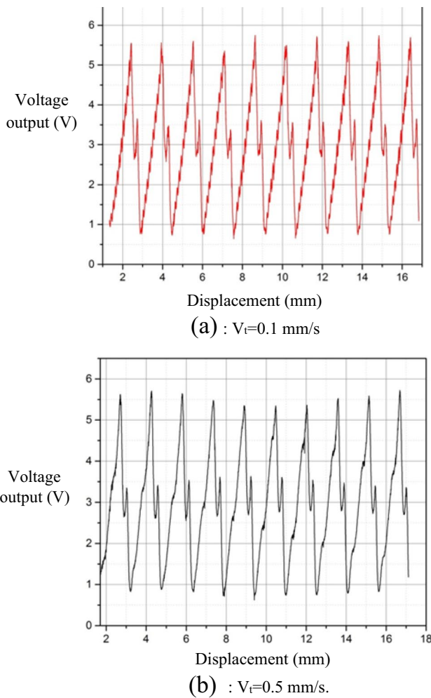
Fig. 18 Voltage output signals of the fiber-optic sensor at two translational velocities
