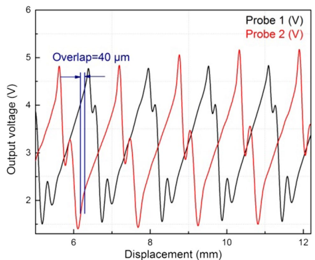
Fig. 20 Signals obtained from the two fiber-optic probes for a coupled motion (translation + rotation)
