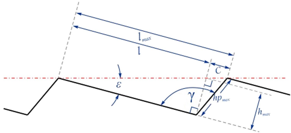
Fig. 11 Geometric parameters of one step in the cones' assembled grating
