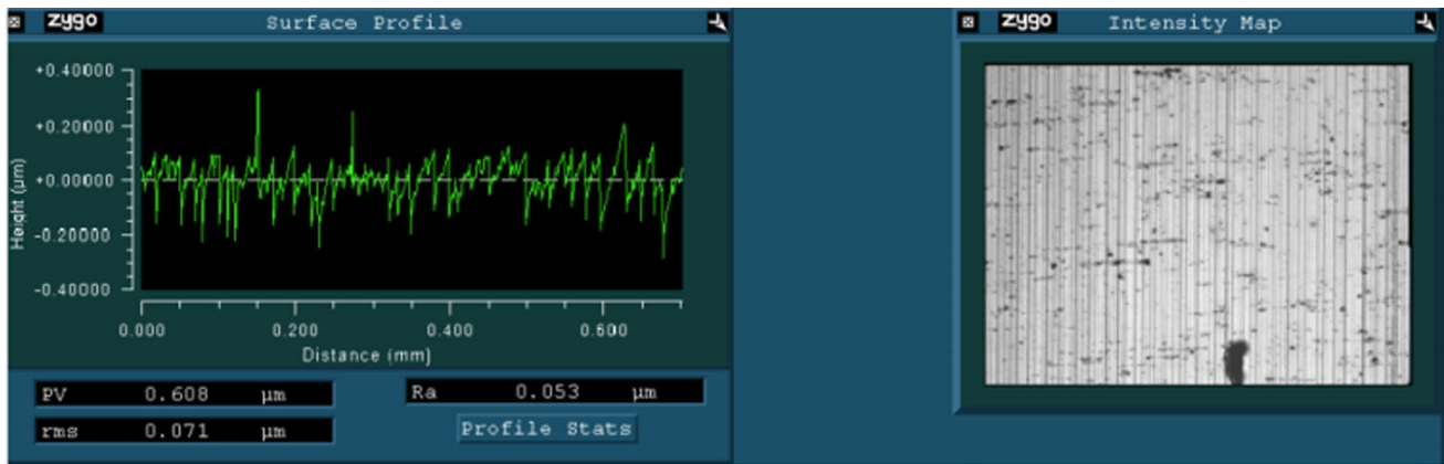
Fig. 16 Surface characteristics
