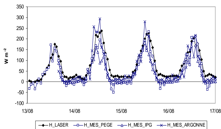
Fig. 5 Validation of the simulated sensible heat flux going out of the top of the voxel ( H\_LASER ) with the data of three measurement sites ( H\_MES ).
