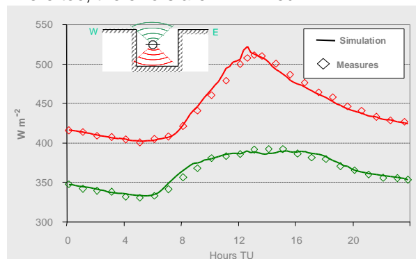
Fig. 4 Validation of the infrared radiation on a horizontal plane at mid height of the canyon
