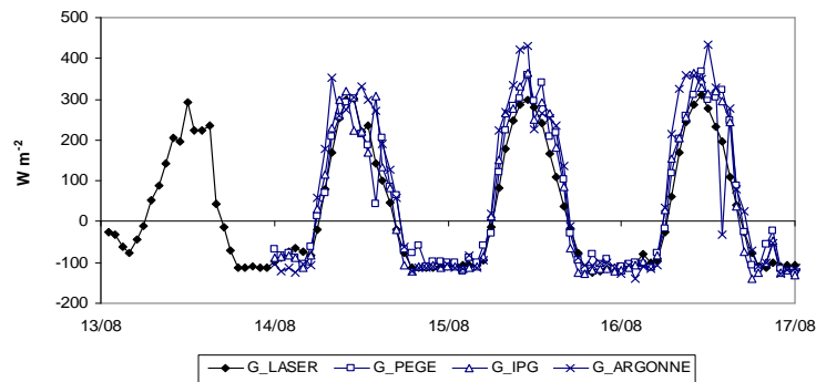
Fig. 6 Validation of the mean ground heat flux simulated for the voxel (G_LASER) with the ground heat flux estimated with the data of three measurement sites.
