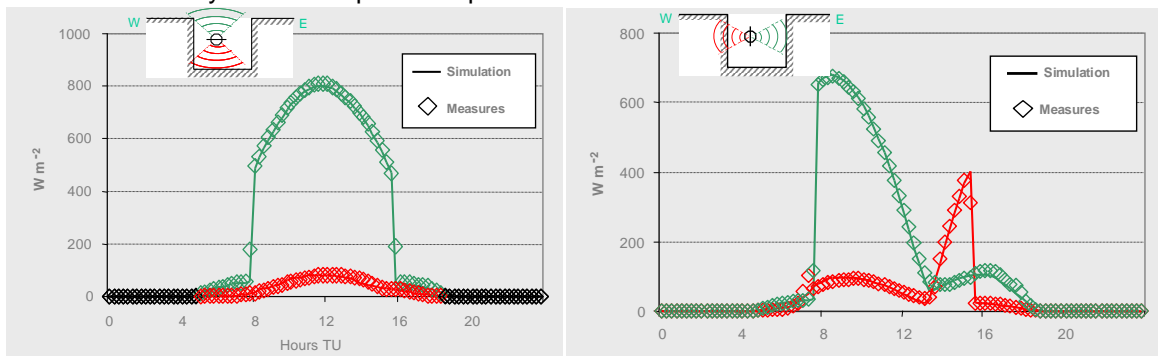
Fig. 3 Validation of the horizontal (left) and vertical (right) global radiation at mid height of the canyon
