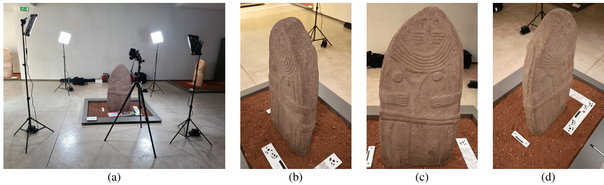
Figure 2. (a) General view of the photogrammetry setup to digitize in 3D a “statue-menhir”. (b-c-d) Three images taken from different viewpoints, under a fixed diffusive lighting.
