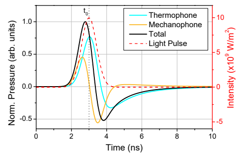
FIG. 1. Left axis: pressure time evolution in water at r = R_{gnc} + 5 nm for \tau_L = 1 ns, \mathcal{R} = 1 \times 10^{-7} m 2 K/W. The curves are normalized to the total pressure maximum. Right axis: I(t) (red dashed curve).
