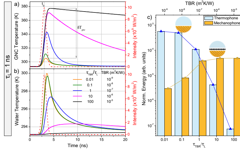
FIG. 2. Laser pulse: \tau_L = 1 ns. Panels (a,b): temperature time evolution, for increasing values of \tau_{TBR}/\tau_L and the corresponding TBR values, in the GNC ( r = 0 nm): panel (a); in proximal water ( r = R_{gnc} + 5 nm): panel (b). Right axis: I(t) (red dashed line) maximized at the time t_0 . \delta T_{gnc} : difference between the GNC peak temperatures between the cases of \tau_{TBR}/\tau_L \sim 100 and 0.01. Panel (c): normalized mechanical energy generated in water by the thermophone and the mechanophone effects for different \tau_{TBR}/\tau_L (bottom axis) and the corresponding TBRs (top axis). The ratios \tau_{TBR}/\tau_L are rounded to the first significant figure. Values for Au/water and graphene-functionalized Au/water interface are identified by the two round sketches.
