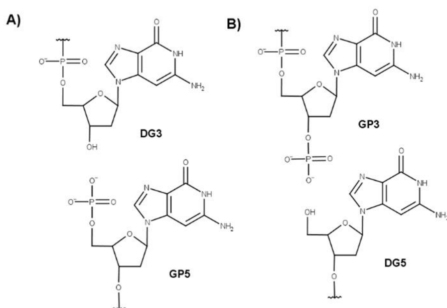
Figure 1. (A) Canonical and (B) non-canonical strand break damages occurring in the phosphodiester -O-P(O 2 )-O- bond of a nucleic acid.
