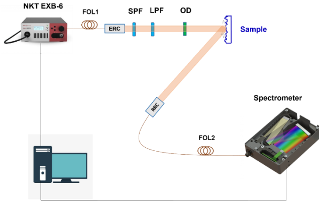
Fig. 3: Schematic representation of the instantaneous spectro-scatterometer ([NKT EXB-6: super-continuum laser source; FOL1: fiber optic link 1; ERC: emission reflective collimator; SPF : short-pass filter ; LPF : long-pass filter ; OD: Optical density filter; RRC: receiving reflective collimator ; FOL2 : fiber optic link 2)
