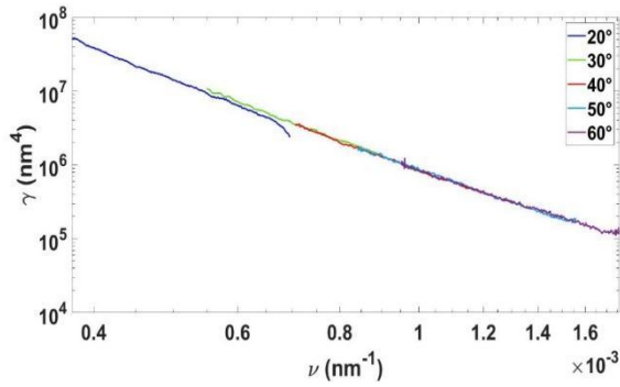
Fig. 6 : Roughness spectra measured for the silicon wafer in different bandwidths, that is, for different positions of the detector
