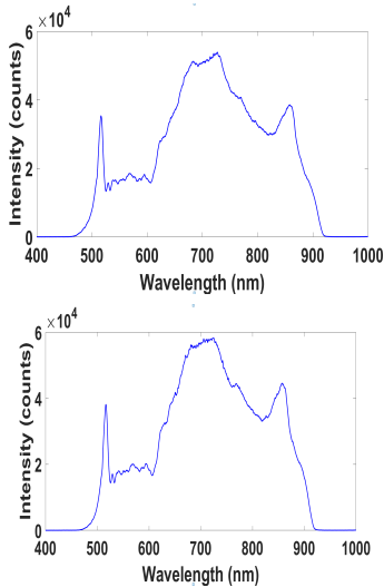
Fig. 4 : White signals measured by the spectro-scatterometer after scattering on the silicon sample (left, integration time is 900 ms) and on the lambertian sample (right, integration time is 8 ms) for a detector placed at 30^\circ .
