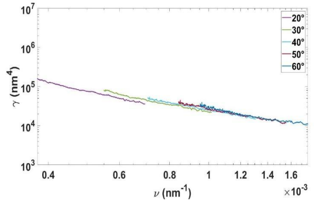
Fig. 7 : Roughness spectra measured for the Al sample in different bandwidths, that is, for different positions of the detector
