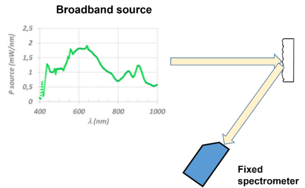
Fig. 2: draft view of the “spectrometer scatterometer” presented in this work. The incident beam is white light
