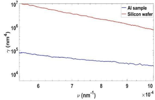
Fig. 5 : Roughness spectra determined for the Si sample and the Al sample
