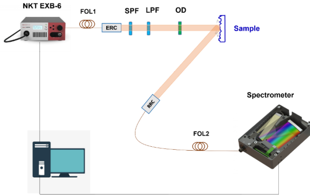
Fig. 3: Schematic representation of the instantaneous spectro-scatterometer ([NKT EXB-6: super-continuum laser source; FOL1: fiber optic link 1; ERC: emission reflective collimator; SPF: short-pass filter; LPF: long-pass filter; OD: Optical density filter; RRC: receiving reflective collimator; FOL2: fiber optic link 2])
