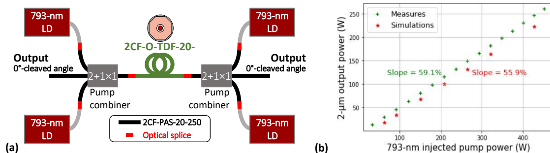
Fig. 1 (a) Schematic of the experimental setup of the Fresnel-cavity configuration of the monolithic single-oscillator thulium-doped fiber laser source. LD: laser diode ; (b) Simulated and measured 2- \mu\text{m} output power versus injected 793-nm pump power.
